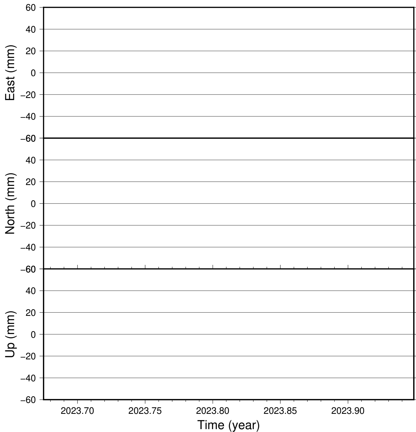
HAMR time series (IGS 2014), last 100 days
