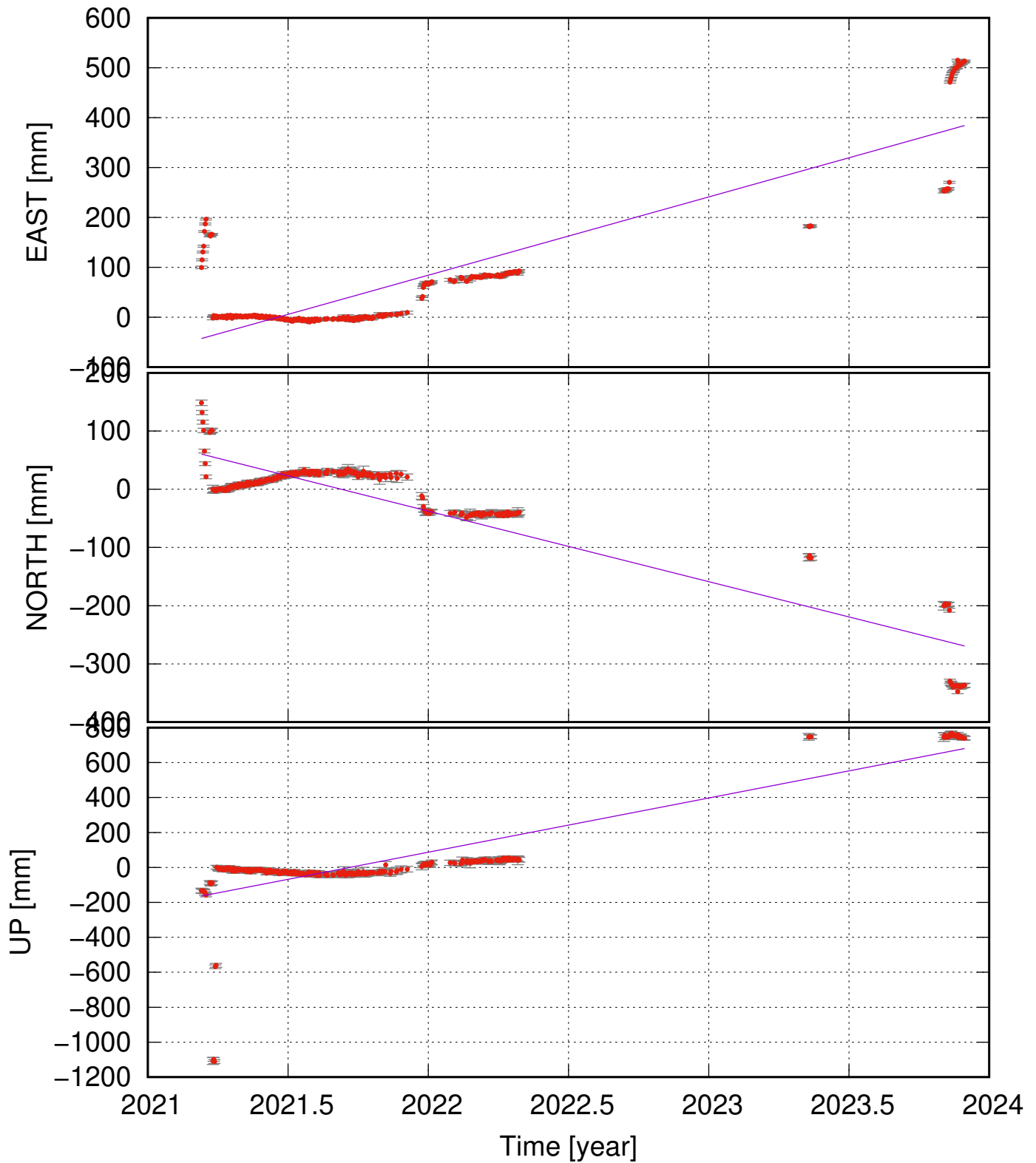
HAMD (63.86, -22.20) time series (ITRF 2014) v_e = 156.89 \pm 22.18 ; v_n = -121.12 \pm 13.35 ; v_u = 310.29 \pm 47.84 mm/yr
