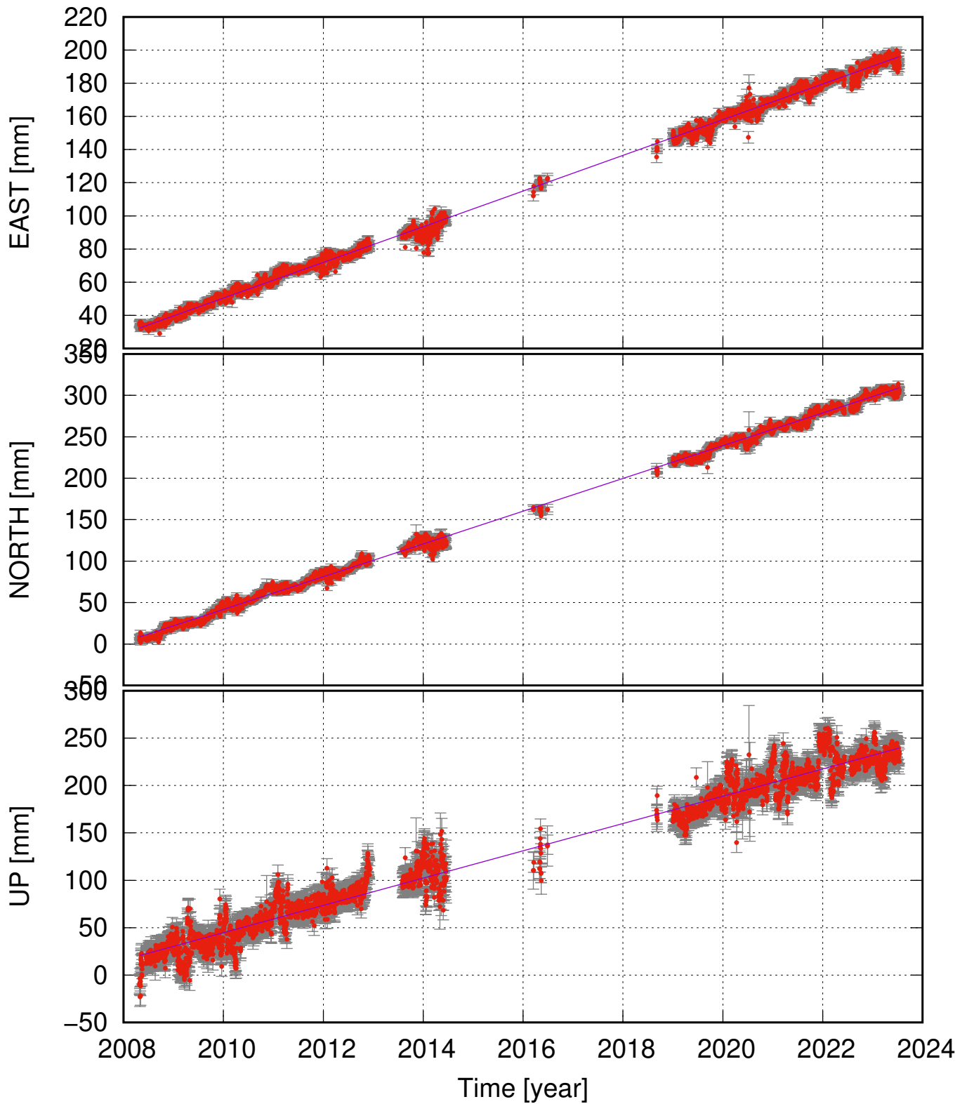
HAHV (64.95, -15.81) time series (ITRF 2014) v_e = 10.76 \pm 0.17 ; v_n = 19.76 \pm 0.28 ; v_u = 14.40 \pm 0.84 mm/yr
