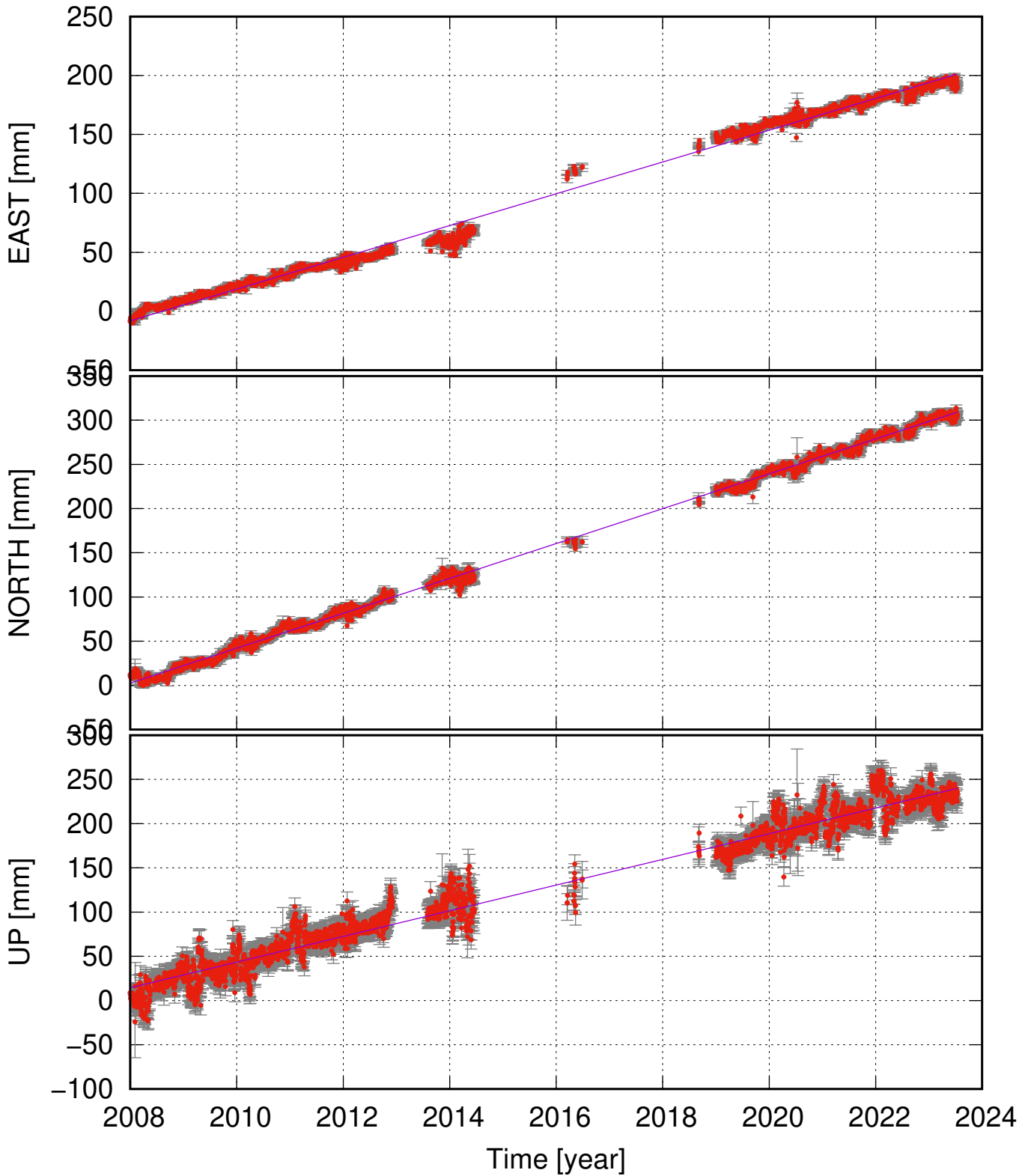
HAHV (64.95, -15.81) time series (ITRF 2014) ve = 13.48 ± 0.35; vn = 19.73 ± 0.28; vu = 14.52 ± 0.83 mm/yr
