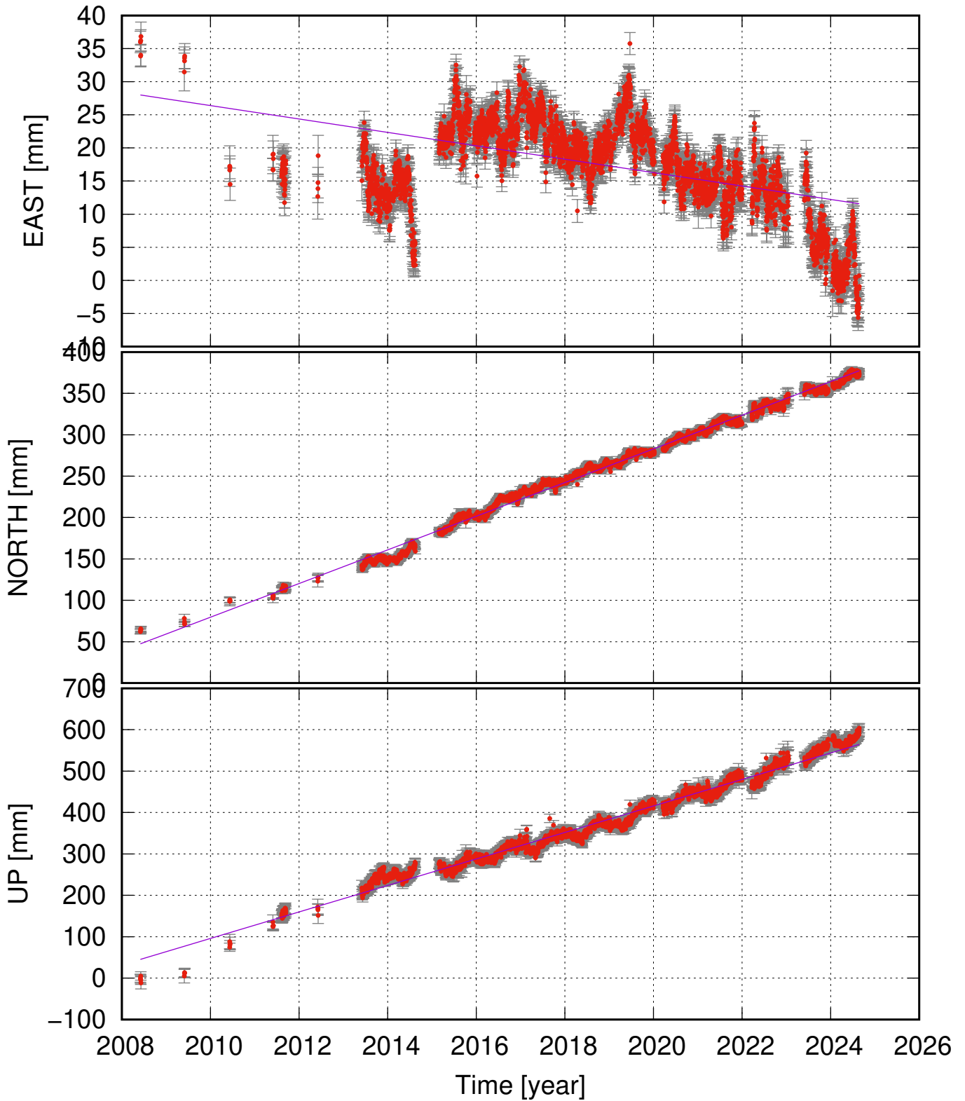
HAFS (64.48, -17.82) time series (ITRF 2014) v_e = -1.01 \pm 0.36 ; v_n = 20.34 \pm 0.36 ; v_u = 32.01 \pm 0.91 mm/yr
