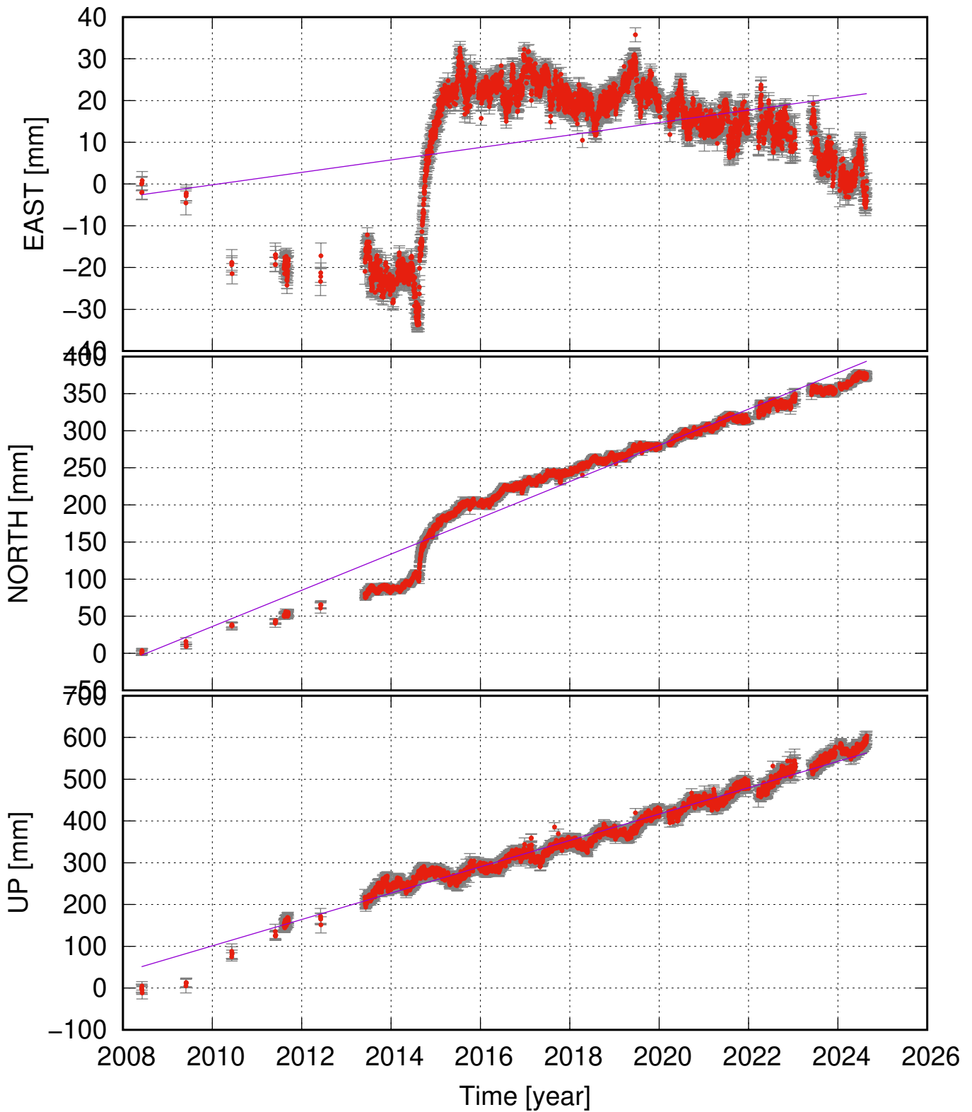
HAFS (64.48, -17.82) time series (ITRF 2014) v_e = 1.49 \pm 0.89 ; v_n = 24.41 \pm 1.27 ; v_u = 31.54 \pm 0.95 mm/yr
