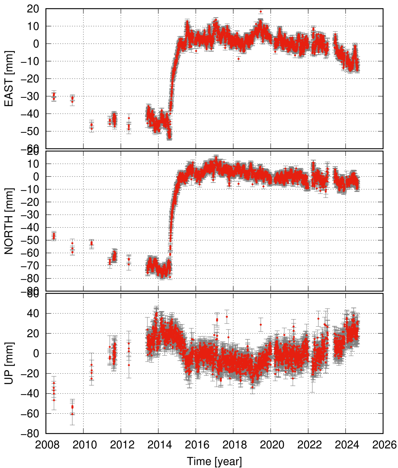
HAFS detrended and seasonal signal removed
