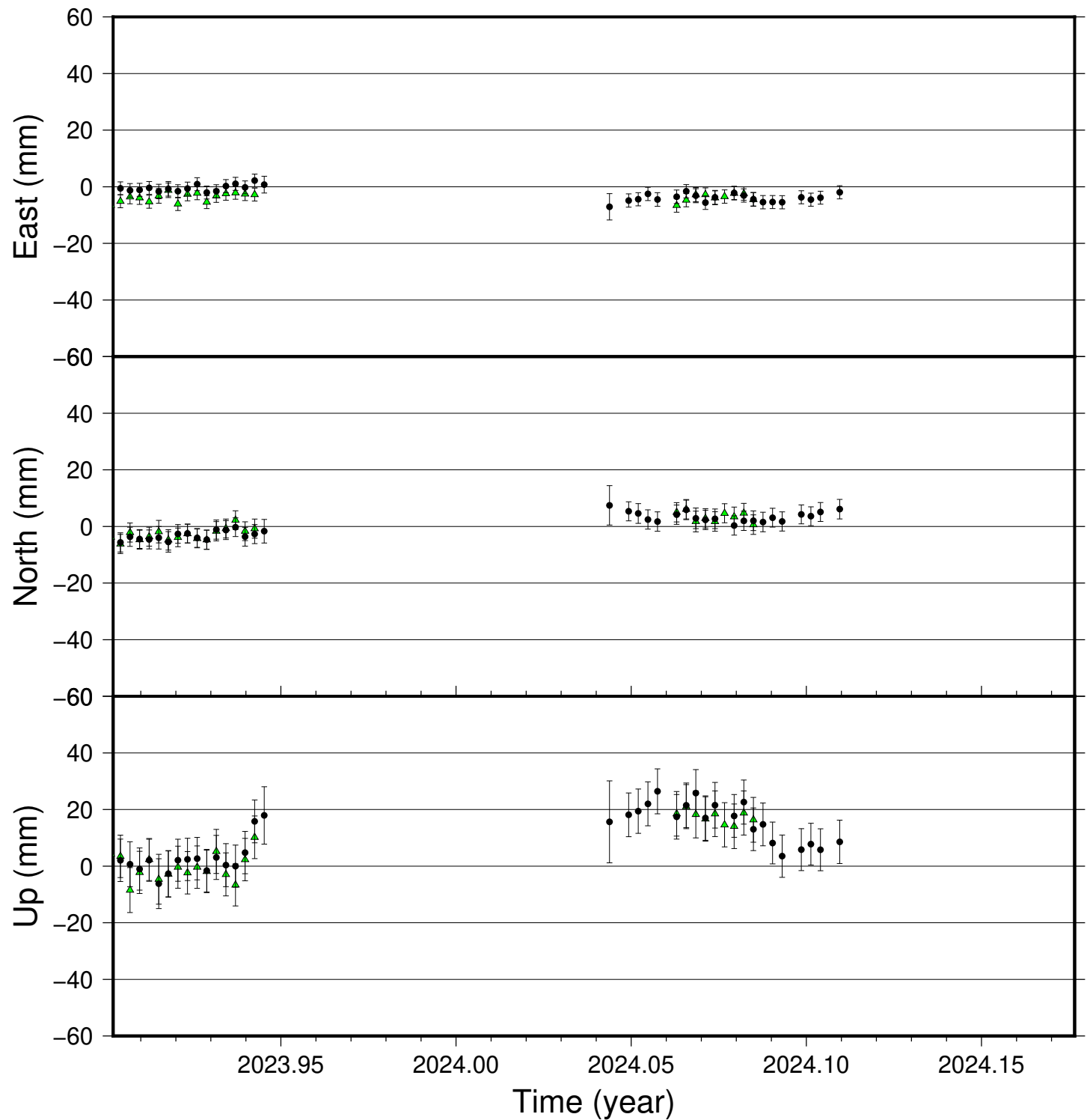
HAFS time series (IGS 2014), last 100 days
