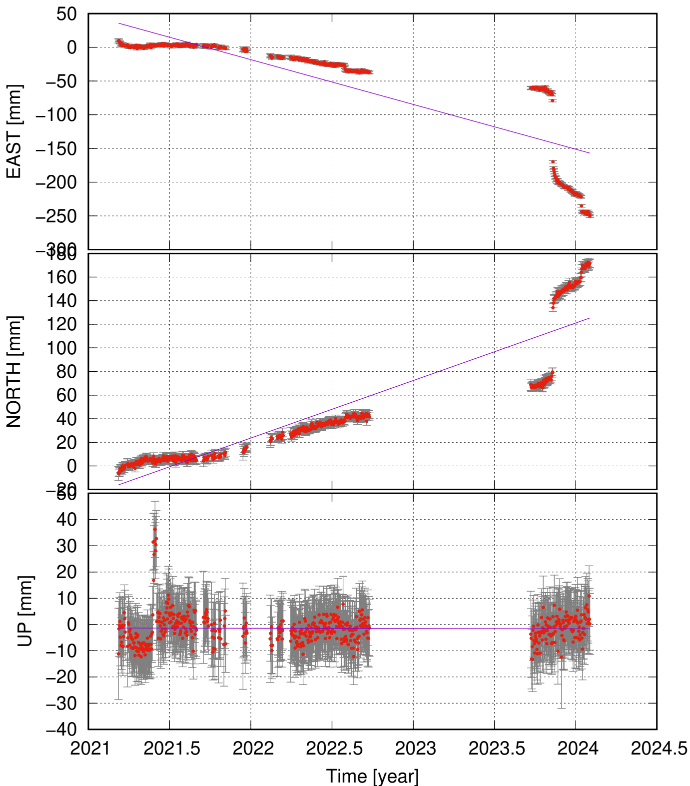
HAFC (63.93, -22.68) time series (ITRF 2014) v_e = -66.44 \pm 13.60 ; v_n = 48.70 \pm 7.07 ; v_u = -0.10 \pm 2.00 mm/yr
