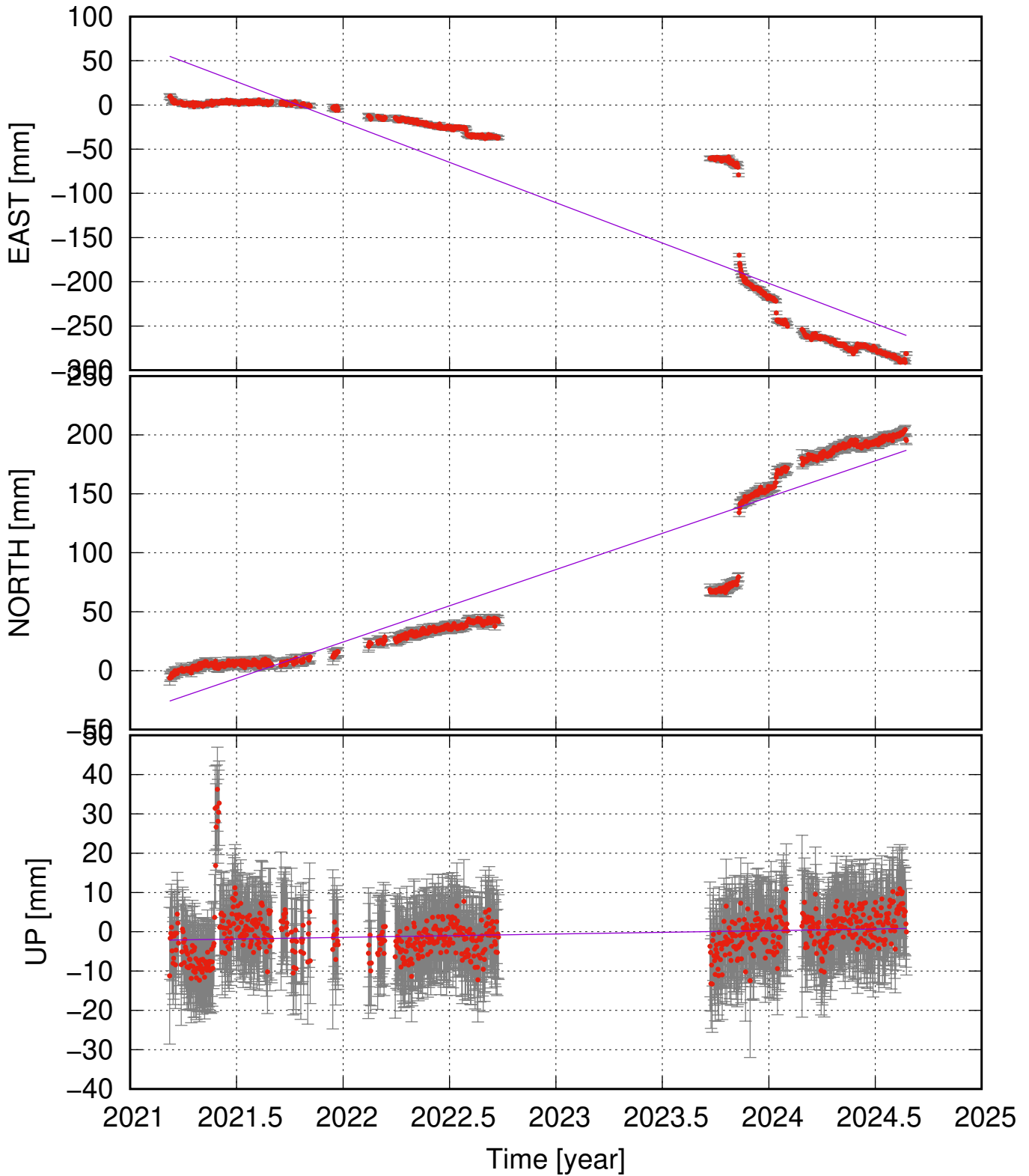
HAFC (63.93, -22.68) time series (ITRF 2014) v_e = -91.25 \pm 12.84 ; v_n = 61.51 \pm 6.69 ; v_u = 0.86 \pm 1.59 mm/yr
