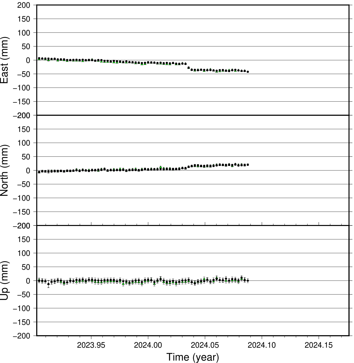
H AFC time series (IGS 2014), last 100 days
