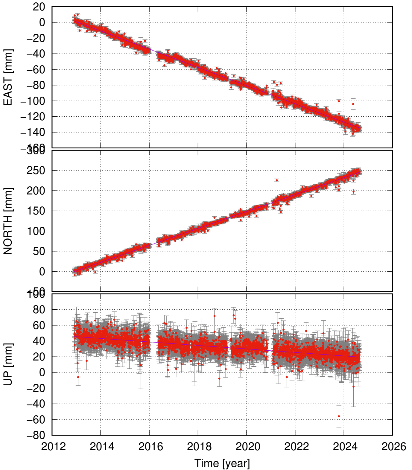
GUSK (64.89, -23.92) time series (ITRF 2014) v_e = -11.61 \pm 0.21 ; v_n = 20.93 \pm 0.28 ; v_u = -2.23 \pm 0.57 mm/yr
