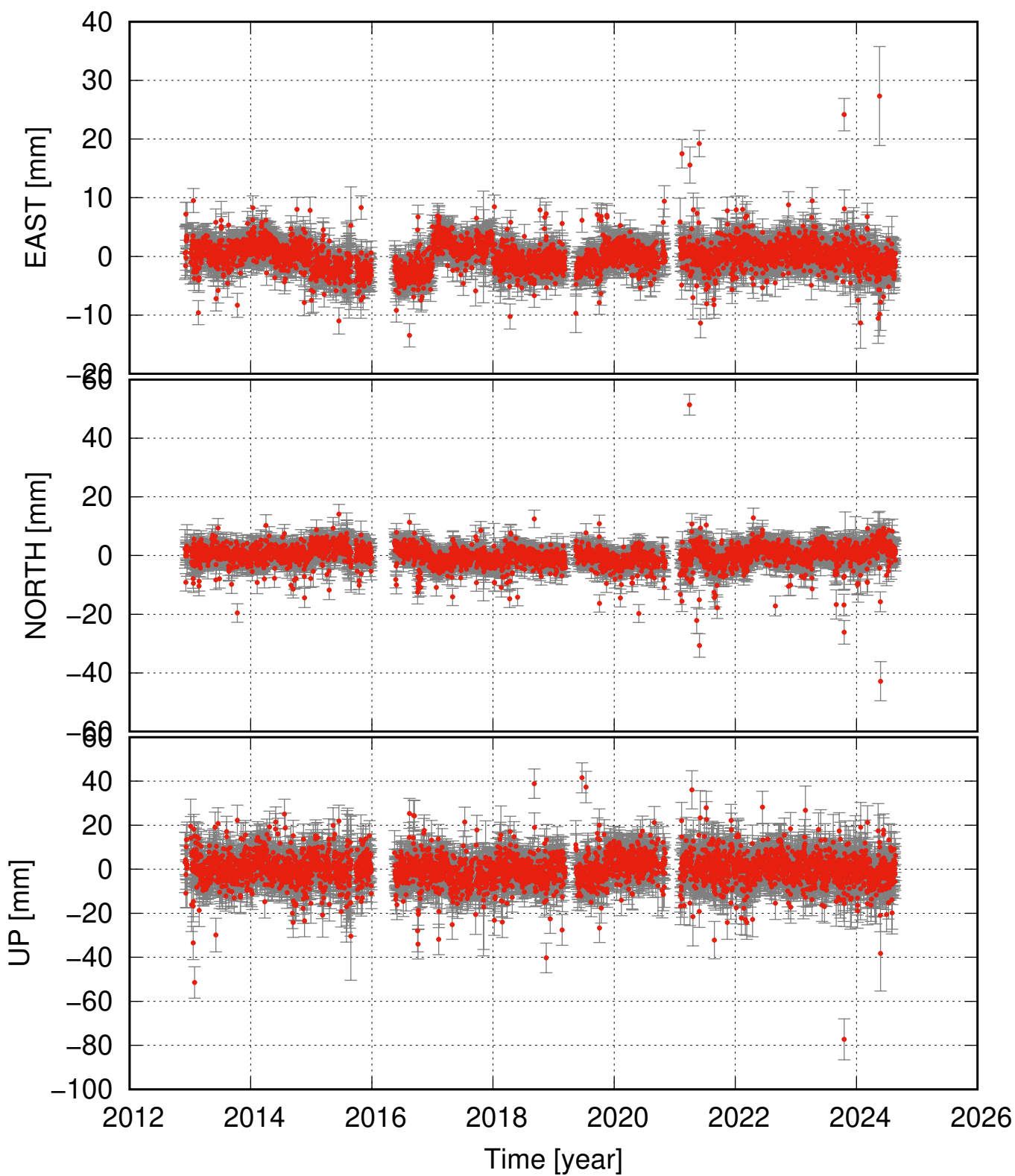
GUSK residual time series (some major events removed as well)
