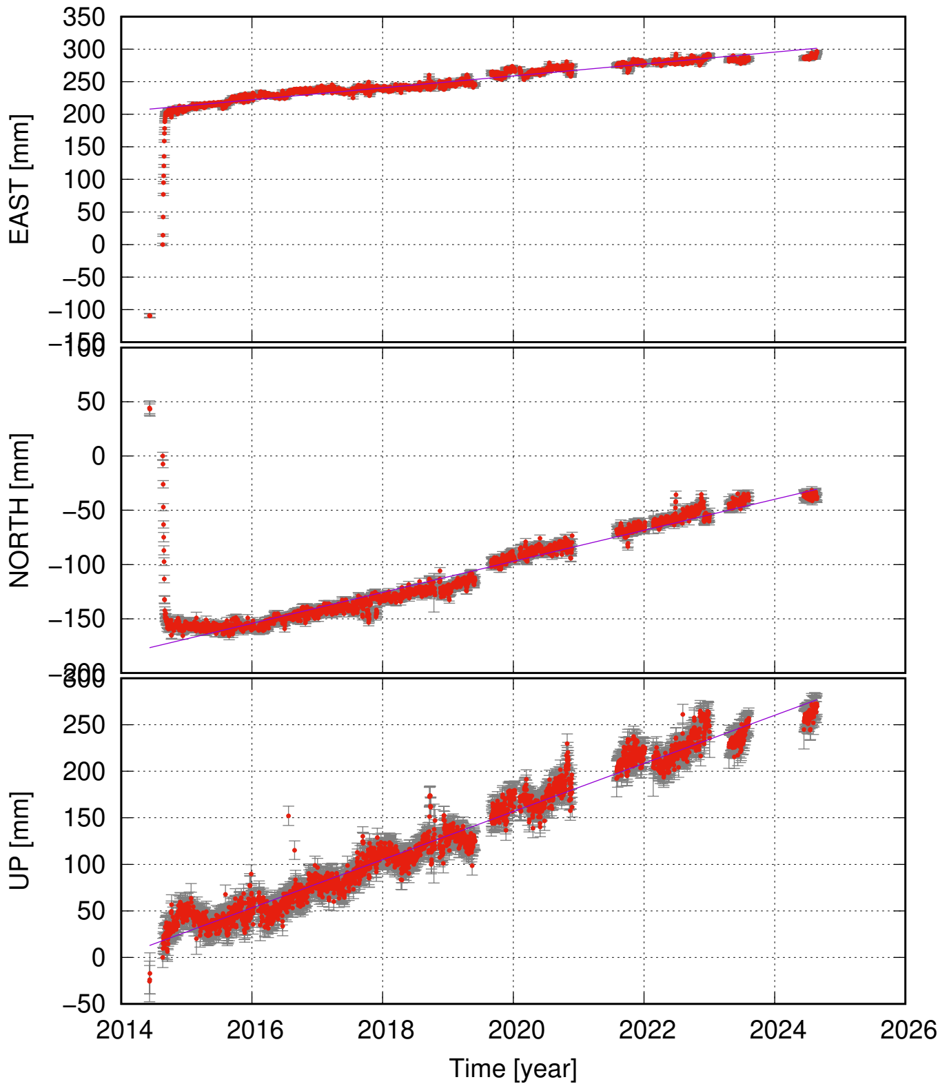
GSIG (64.68, -16.68) time series (ITRF 2014) ve = 9.15 +- 1.39; vn = 14.29 +- 1.20; vu = 25.86 +- 1.18 mm/yr
