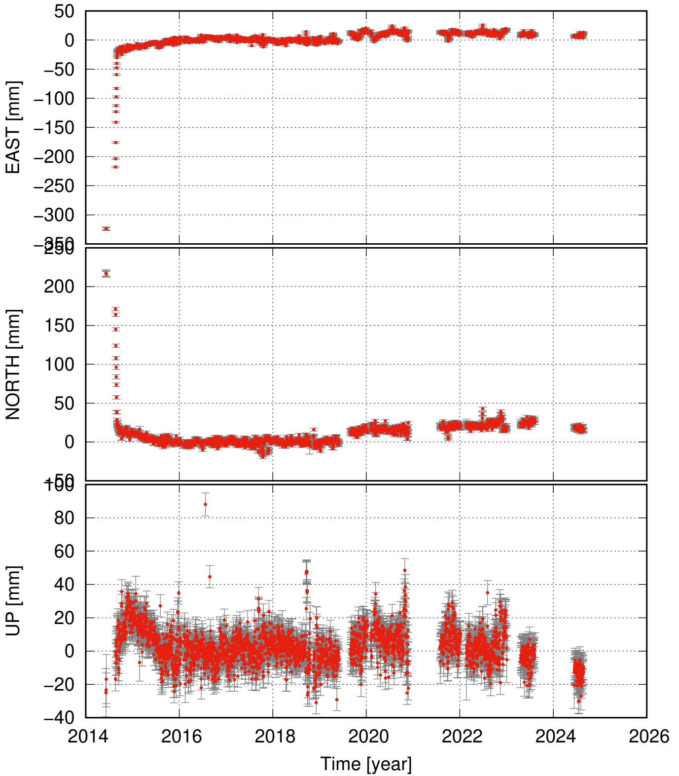
GSIG detrended and seasonal signal removed
