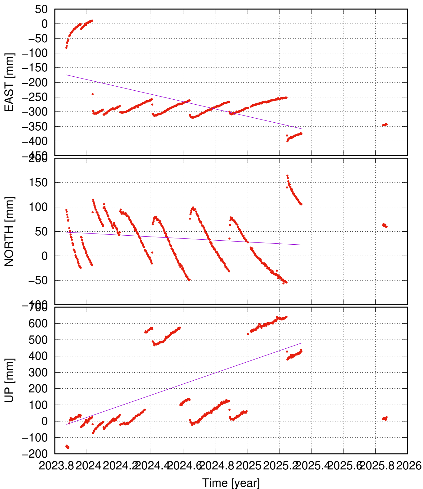
GRVV ( , ) time series (IGb20) ve = +- ; vn = +- ; vu = +- mm/yr
