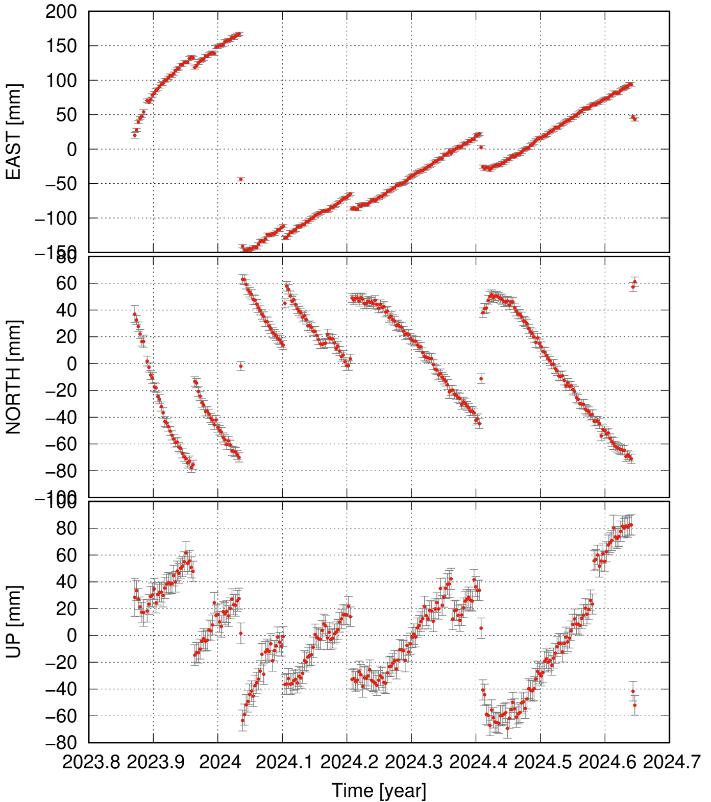
GRVV residual time series (some major events removed as well)
