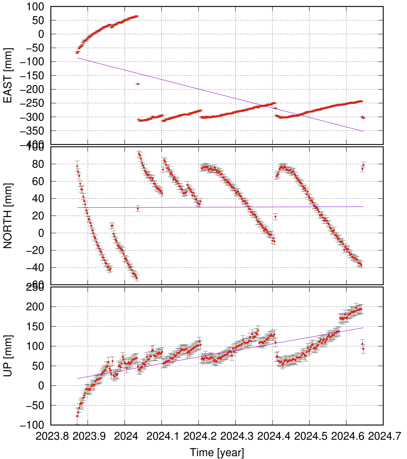
GRVM (63.84, -22.43) time series (ITRF 2014) ve = -343.50 ± 127.53; vn = 1.38 ± 49.30; vu = 166.15 ± 36.60 mm/yr
