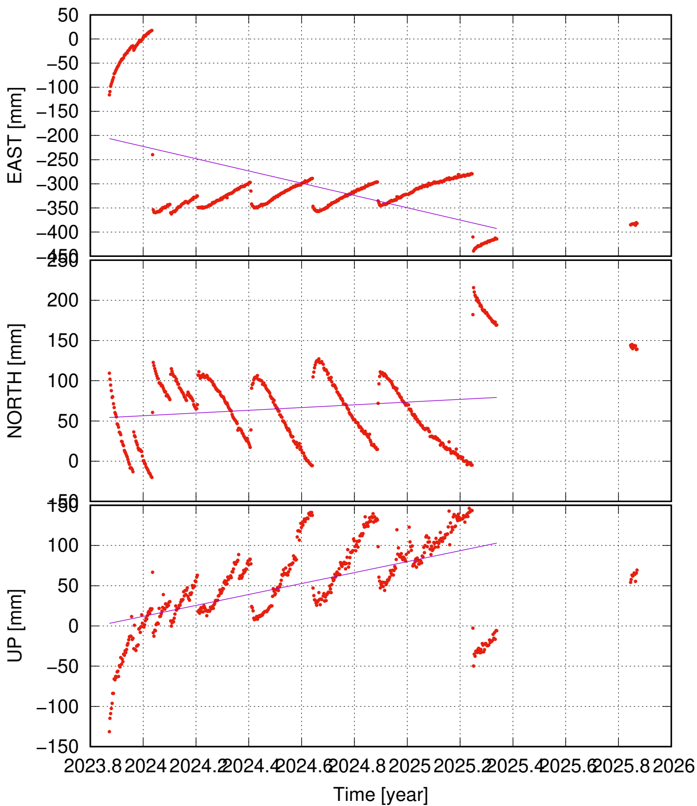
GRVM ( , ) time series (IGb20) ve = +- ; vn = +- ; vu = +- mm/yr
