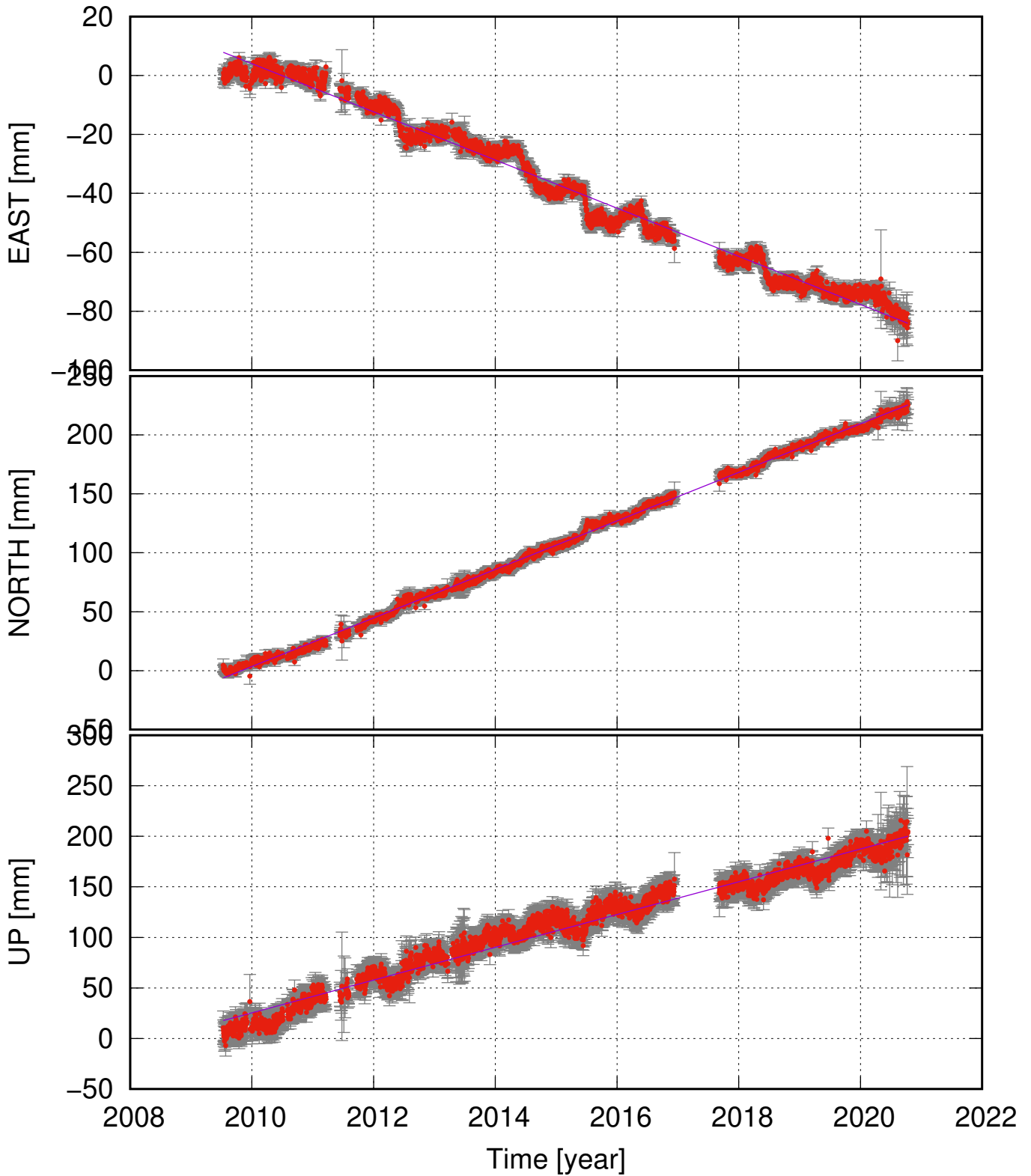
GRVA (64.46, -19.38) time series (ITRF 2014) v_e = -8.18 \pm 0.31 ; v_n = 20.58 \pm 0.25 ; v_u = 16.21 \pm 0.84 mm/yr
