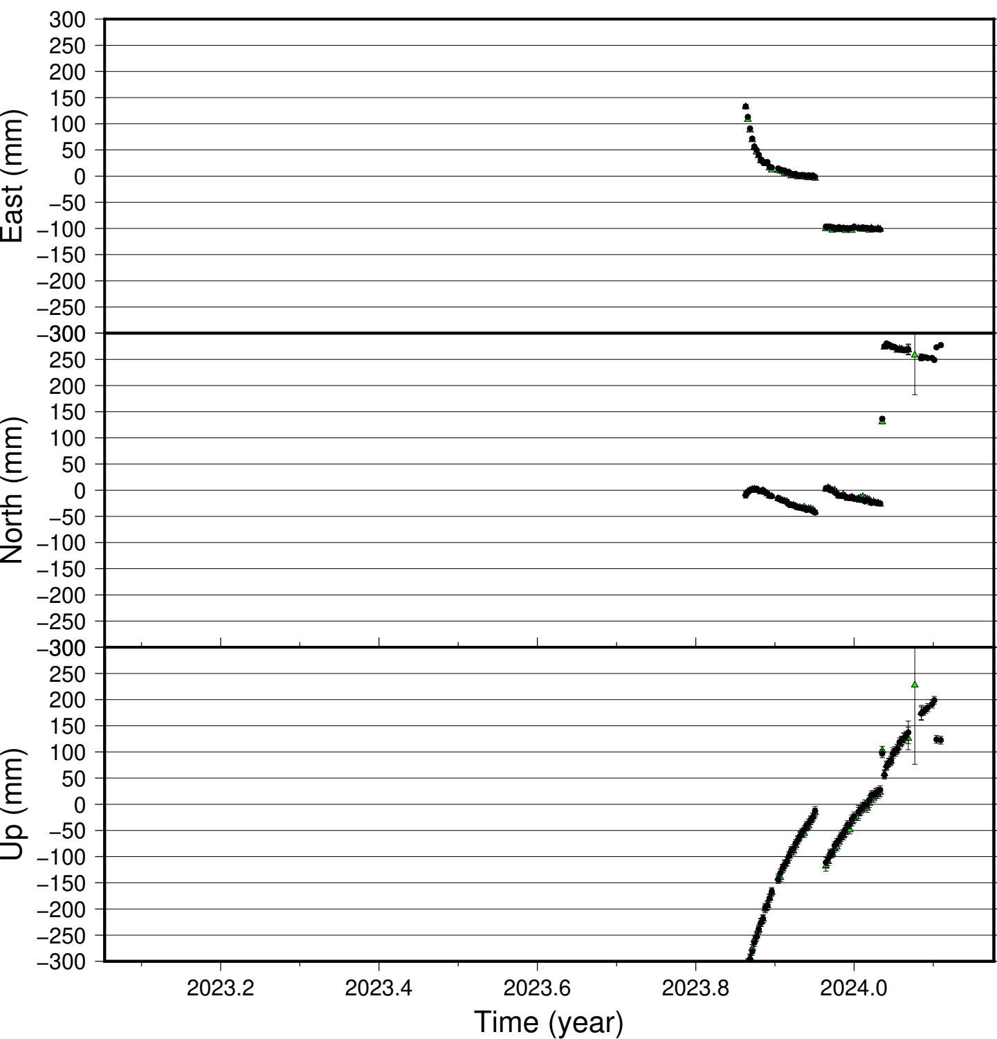
GRIV time series (IGS 2014), last 400 days
