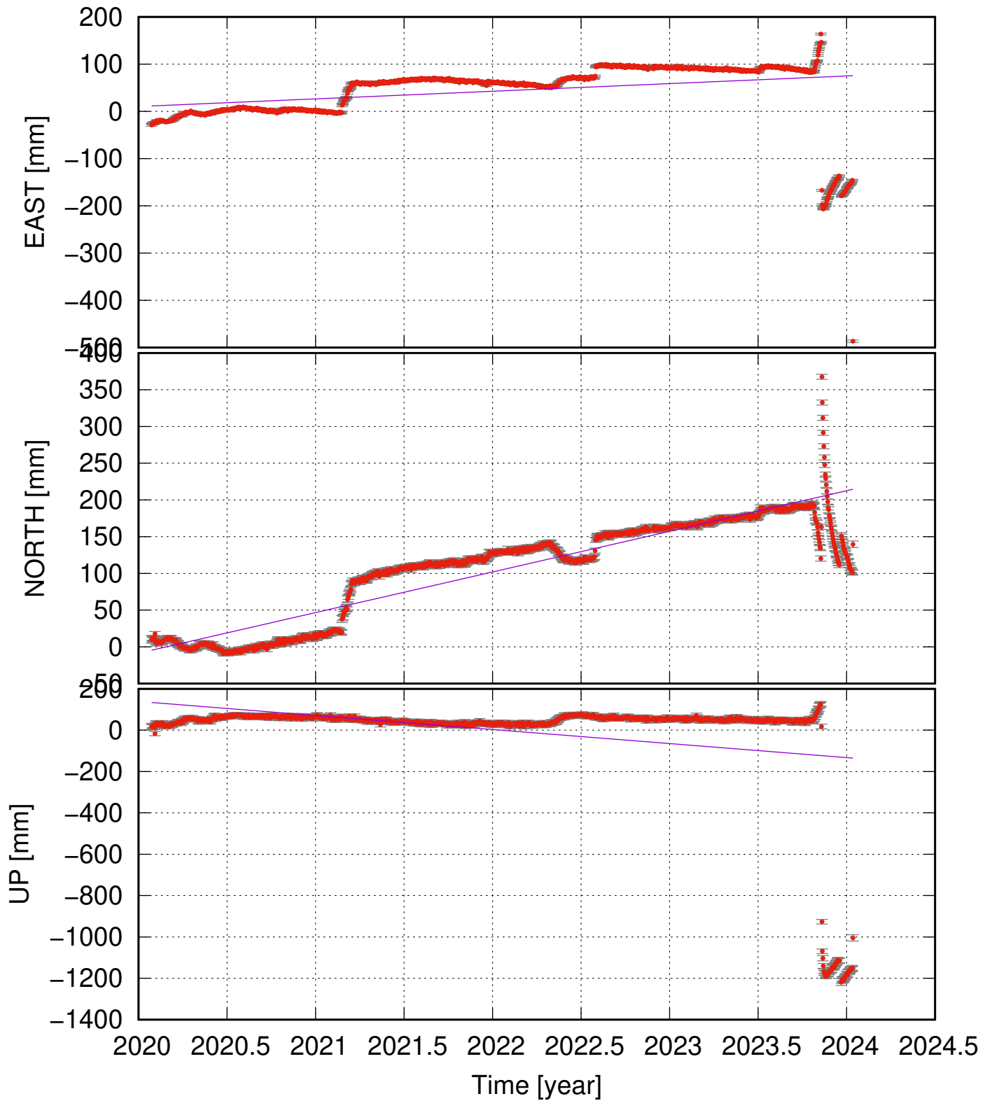
GRIC (63.85, -22.43) time series (ITRF 2014) v_e = 16.10 \pm 14.59 ; v_n = 55.27 \pm 6.65 ; v_u = -67.82 \pm 57.72 mm/yr
