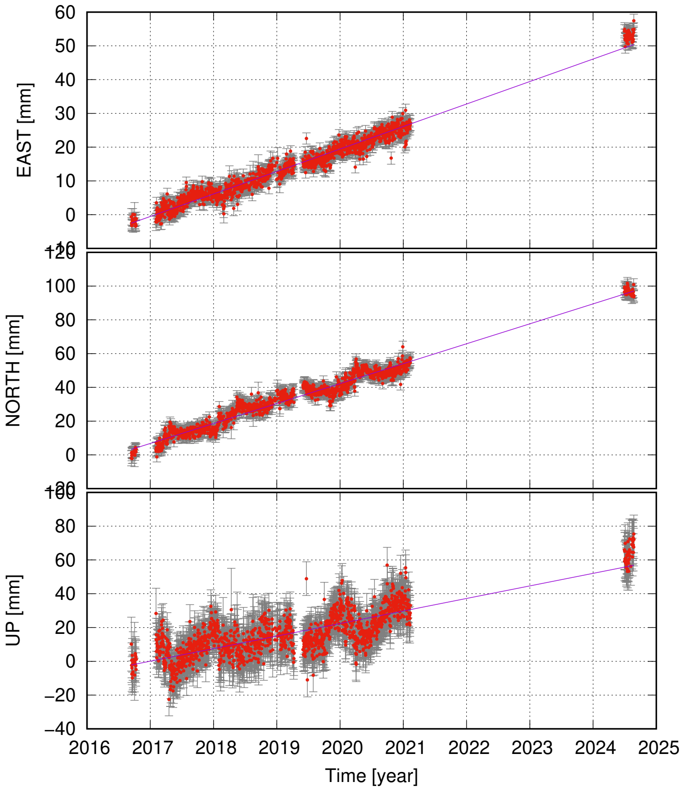
GRFS (63.53, -19.11) time series (ITRF 2014) v_e = 6.66 \pm 0.23 ; v_n = 11.81 \pm 0.42 ; v_u = 7.43 \pm 1.05 mm/yr
