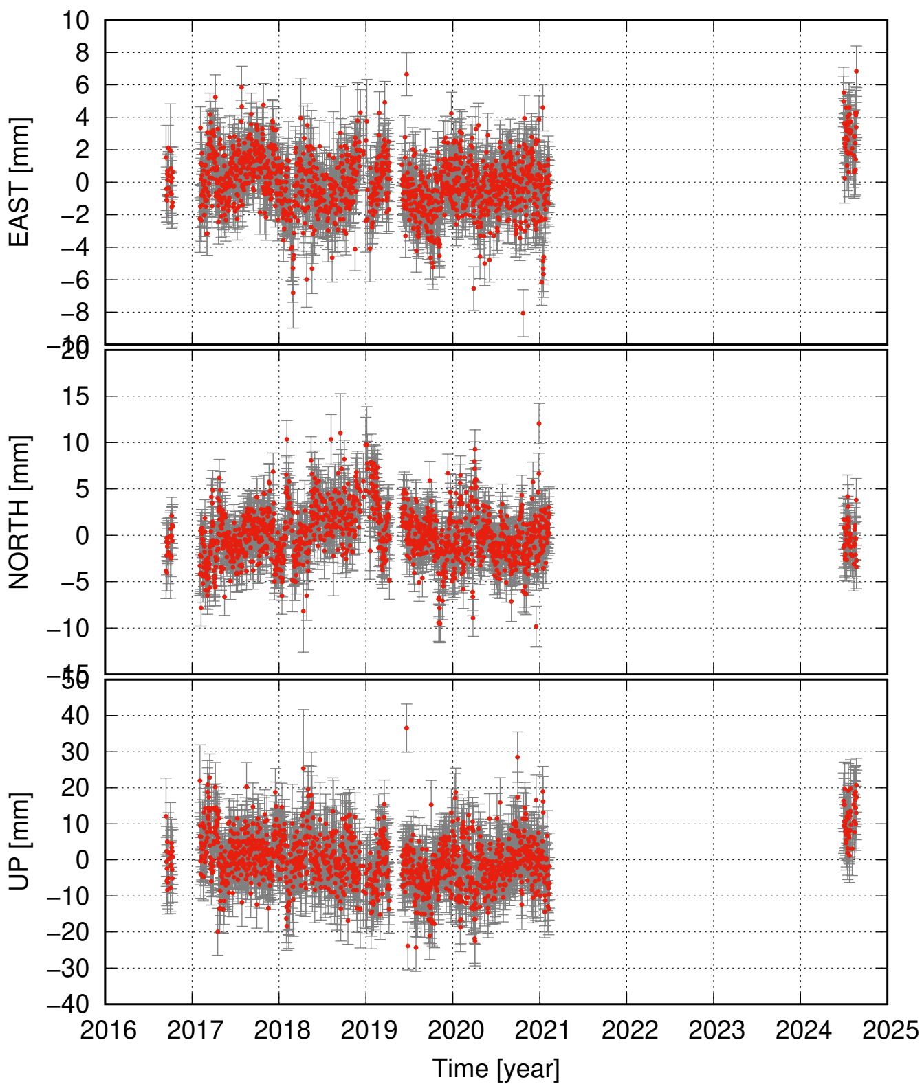
GRFS detrended and seasonal signal removed
