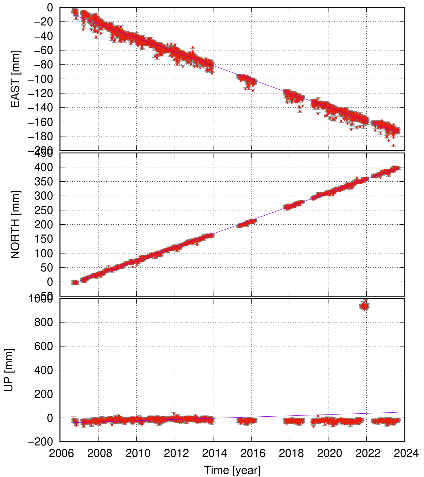
GRAN (65.92, -17.58) time series (ITRF 2014) v_e = -9.69 \pm 0.21 ; v_n = 23.75 \pm 0.18 ; v_u = 5.13 \pm 8.50 mm/yr
