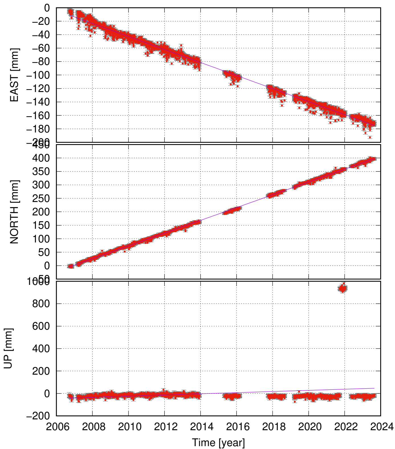
GRAN (65.92, -17.58) time series (ITRF 2014) v_e = -9.69 \pm 0.21 ; v_n = 23.75 \pm 0.18 ; v_u = 5.13 \pm 8.50 mm/yr
