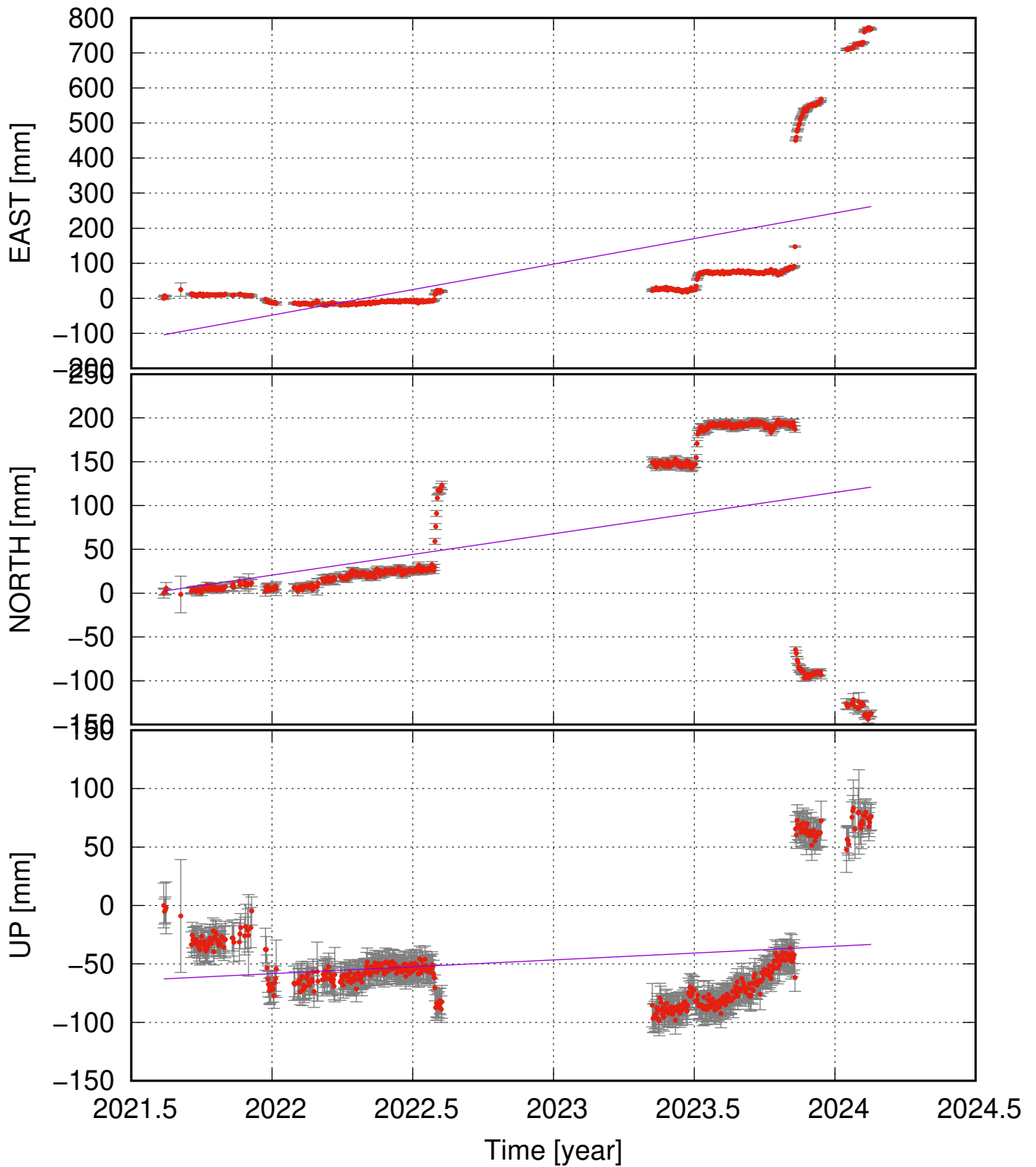
GONH (63.89, -22.27) time series (ITRF 2014) v_e = 145.40 \pm 62.25 ; v_n = 47.17 \pm 36.63 ; v_u = 11.73 \pm 17.39 mm/yr
