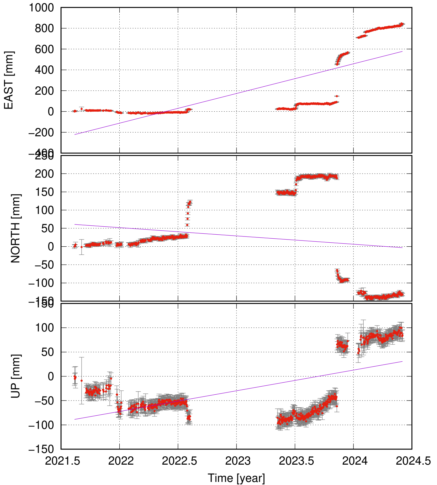
GONH (63.89, -22.27) time series (ITRF 2014) v_e = 285.26 \pm 75.90 ; v_n = -22.82 \pm 41.44 ; v_u = 42.55 \pm 18.84 mm/yr
