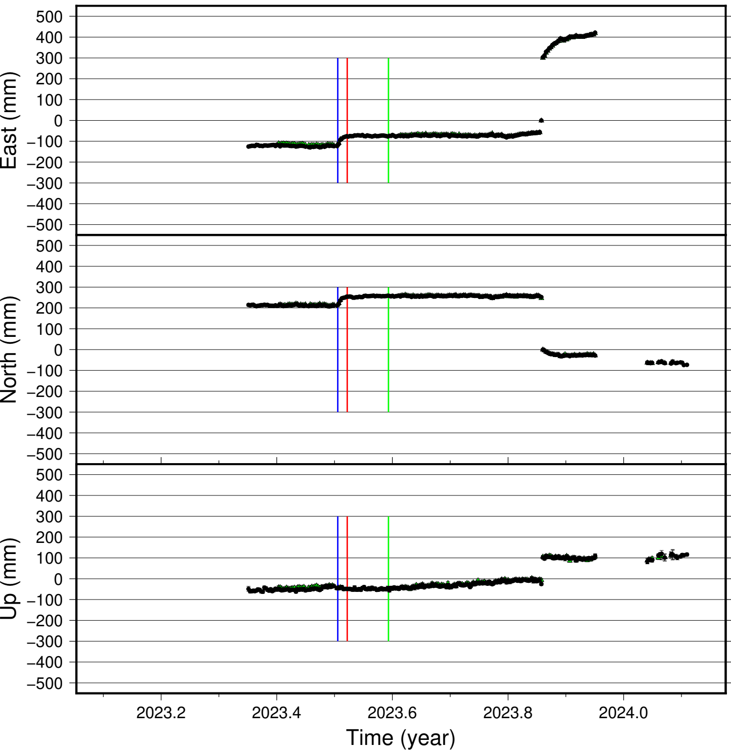
GONH time series (IGS 2014), last 400 days
