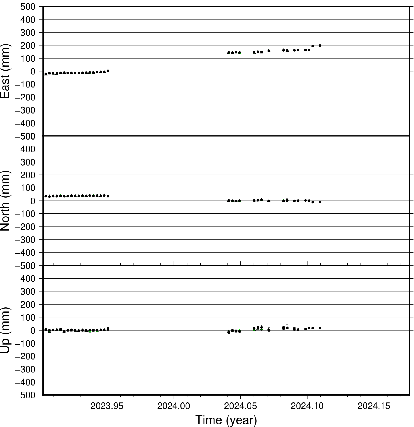
GONH time series (IGS 2014), last 100 days
