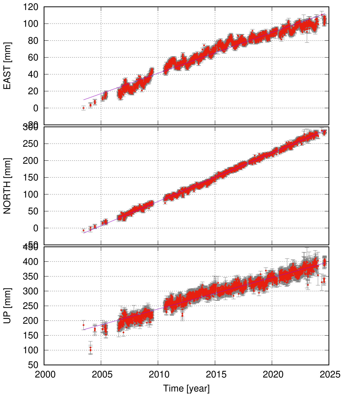
GOLA (63.66, -19.32) time series (ITRF 2014) v_e = 4.83 \pm 0.24 ; v_n = 14.38 \pm 0.19 ; v_u = 10.66 \pm 0.56 mm/yr
