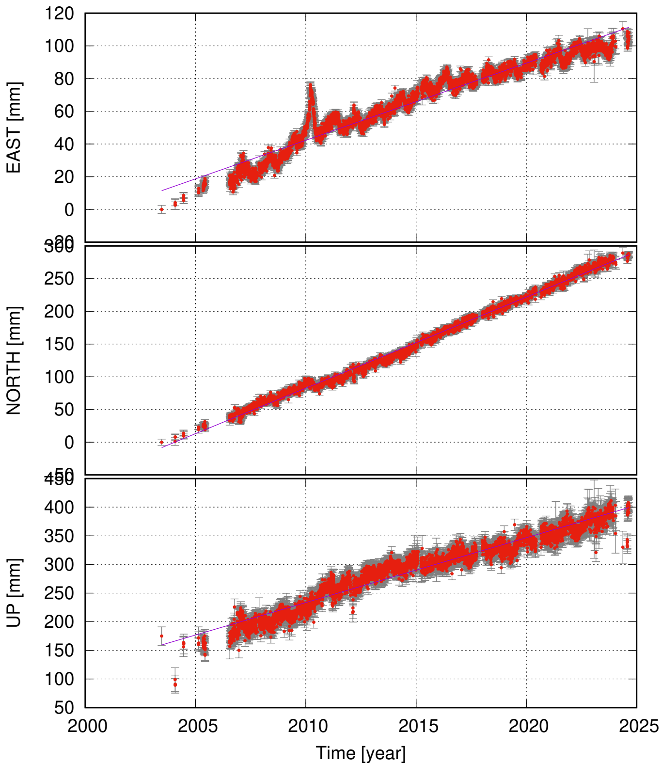
GOLA (63.66, -19.32) time series (ITRF 2014) v_e = 4.72 \pm 0.28 ; v_n = 13.92 \pm 0.24 ; v_u = 11.33 \pm 0.63 mm/yr
