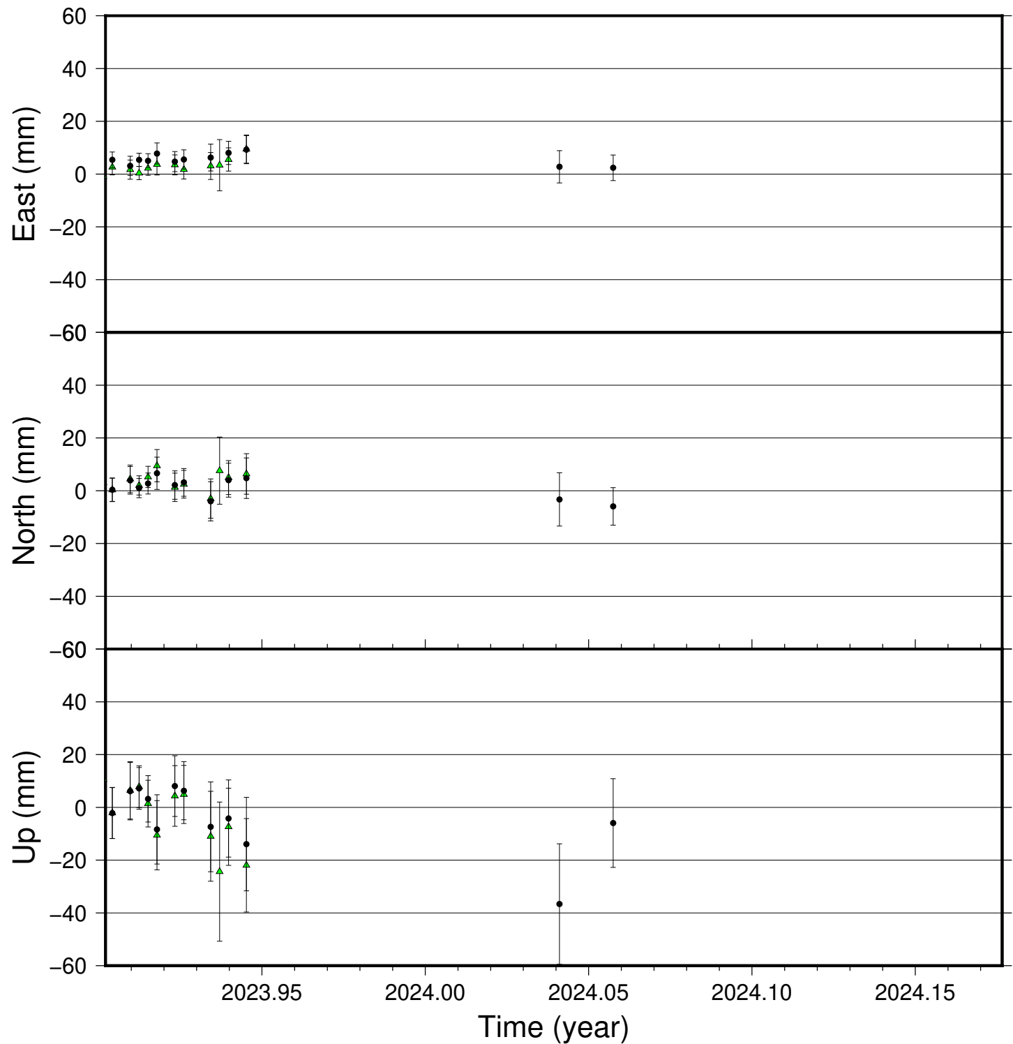
GOLA time series (IGS 2014), last 100 days
