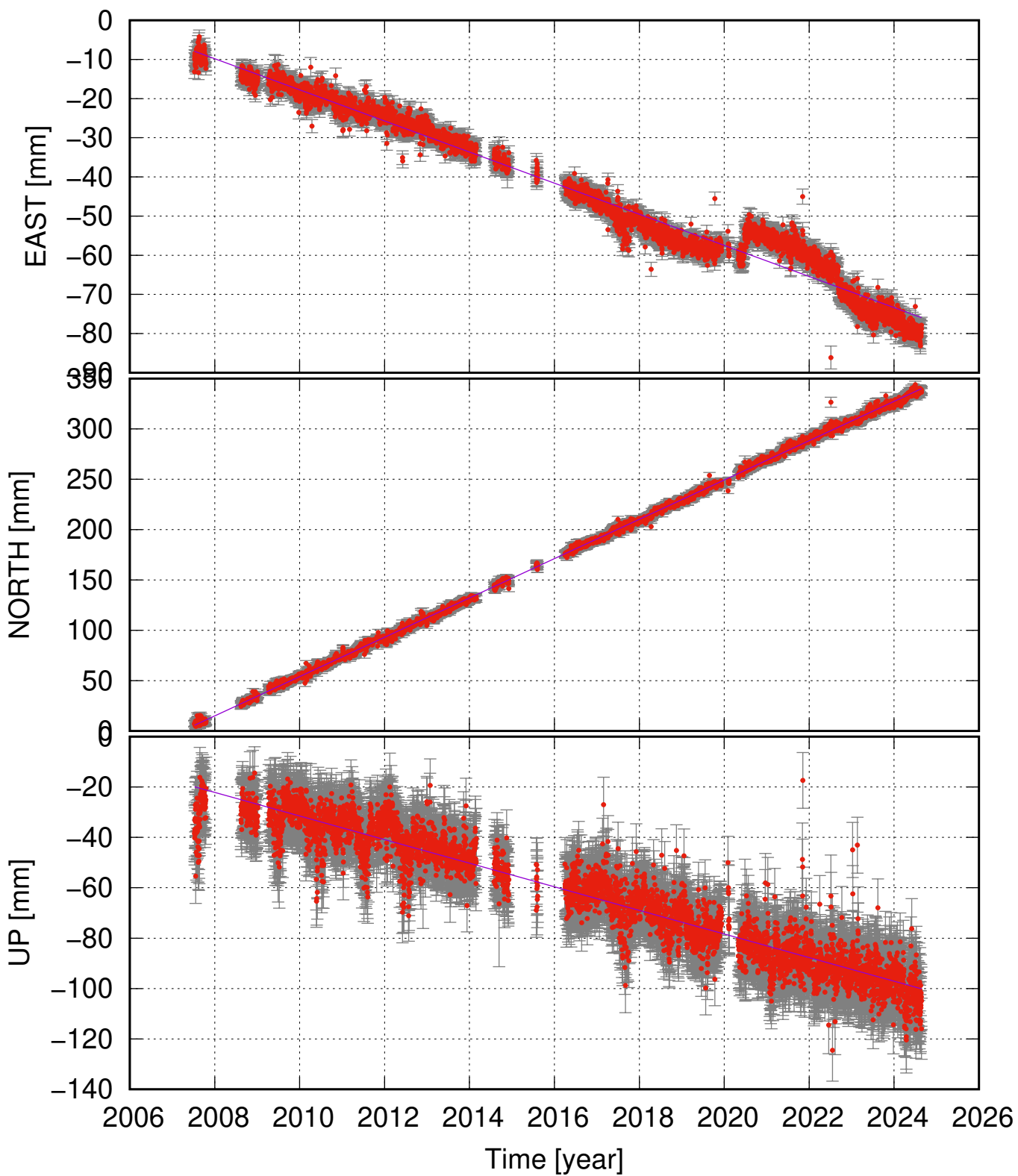
GMEY (66.54, -18.02) time series (ITRF 2014) v_e = -3.97 \pm 0.19 ; v_n = 19.51 \pm 0.13 ; v_u = -4.68 \pm 0.40 mm/yr
