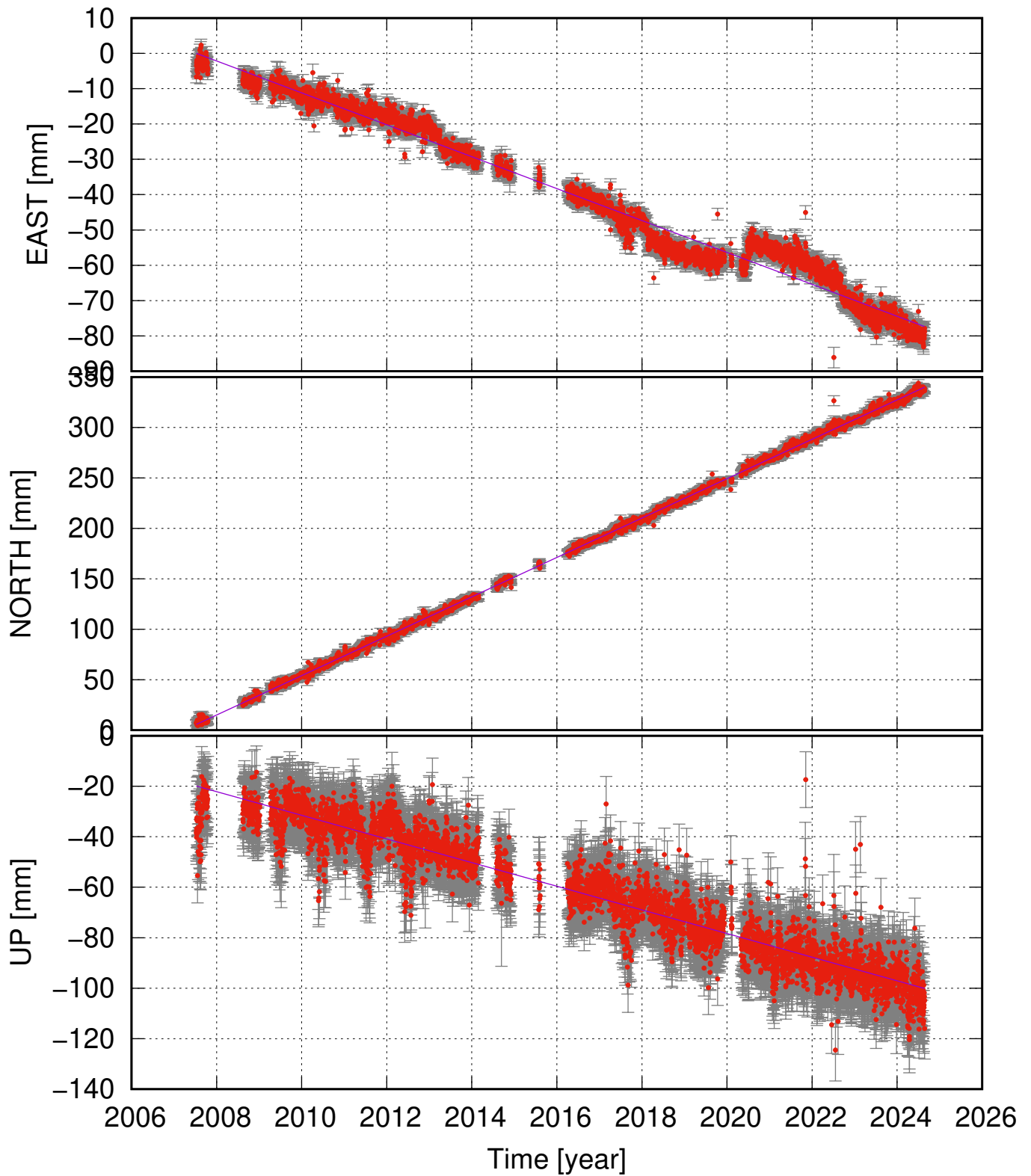
GMEY (66.54, -18.02) time series (ITRF 2014) v_e = -4.52 \pm 0.20 ; v_n = 19.51 \pm 0.13 ; v_u = -4.68 \pm 0.40 mm/yr
