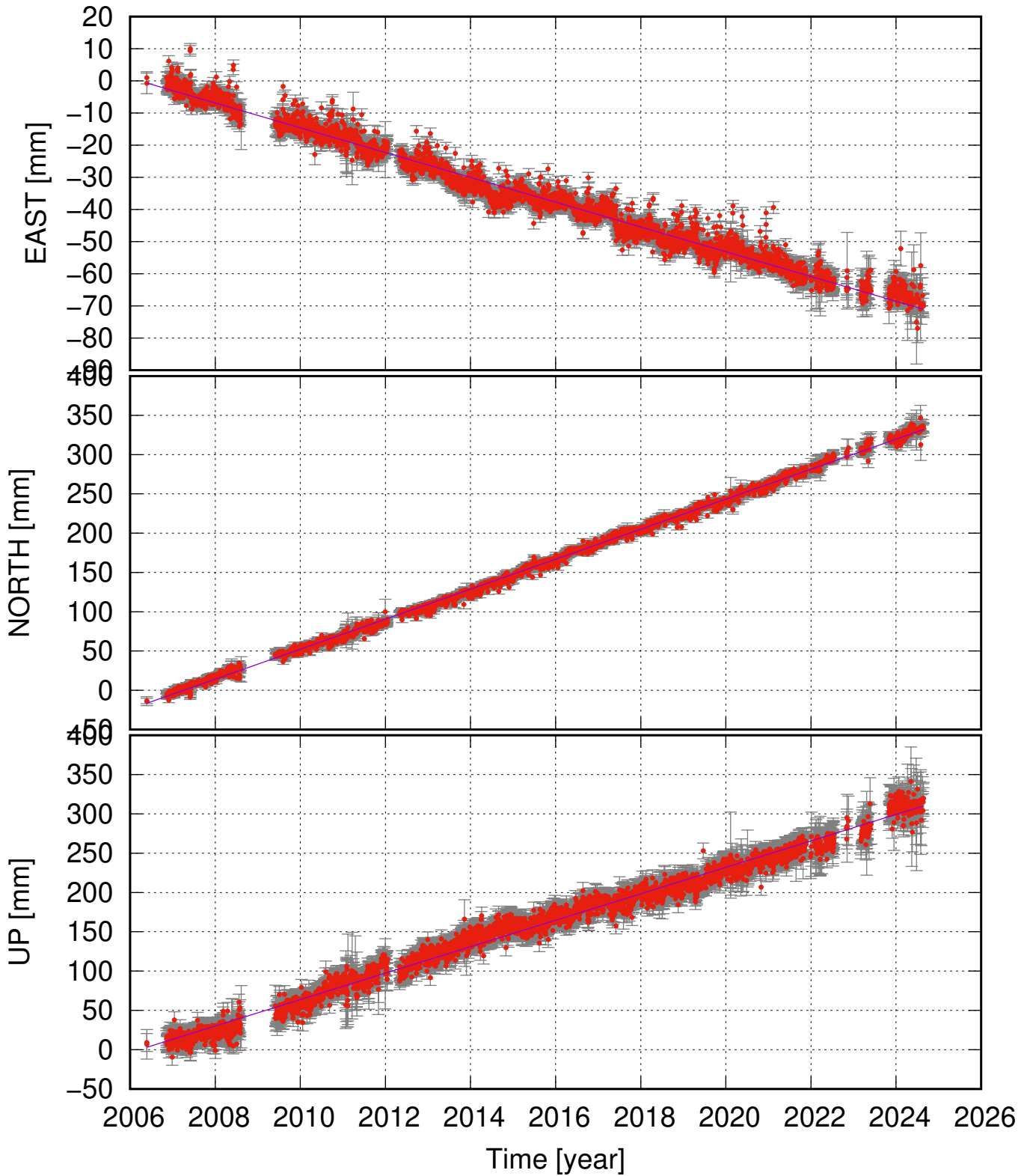
GLER (64.02, -19.80) time series (ITRF 2014) v_e = -3.86 \pm 0.14 ; v_n = 19.09 \pm 0.19 ; v_u = 16.82 \pm 0.48 mm/yr
