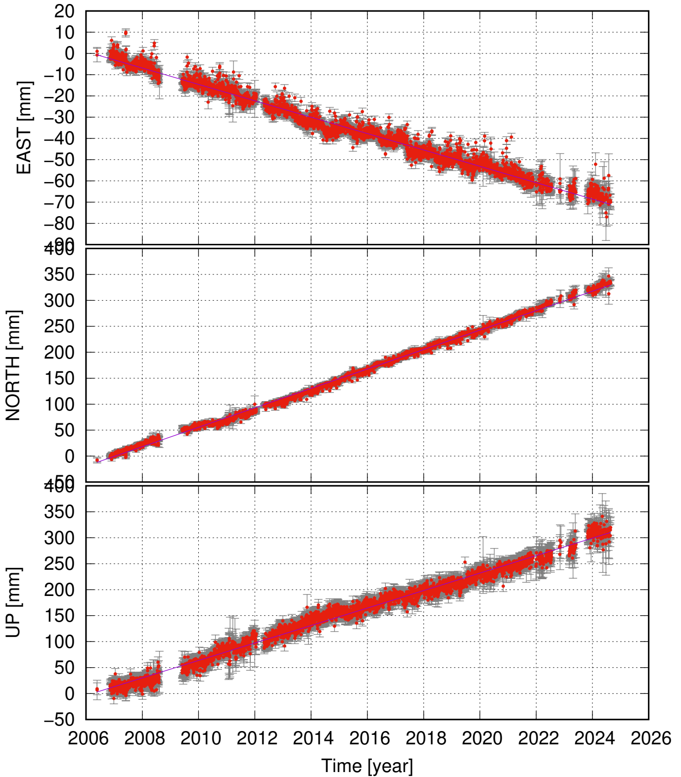
GLER (64.02, -19.80) time series (ITRF 2014) v_e = -3.86 \pm 0.14 ; v_n = 18.71 \pm 0.24 ; v_u = 16.82 \pm 0.48 mm/yr
