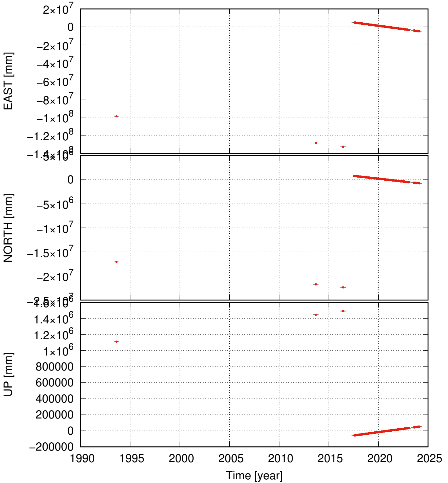
GJOG residual time series (some major events removed as well)
