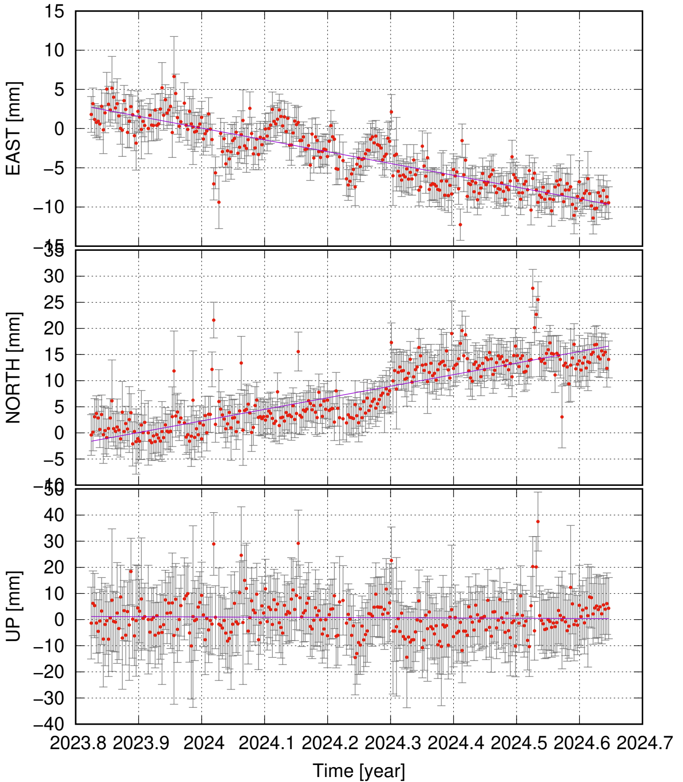
GJFV (66.00, -21.33) time series (ITRF 2014) ve = -15.05 \pm 2.34 ; vn = 22.14 \pm 3.98 ; vu = -1.00 \pm 8.21 mm/yr
