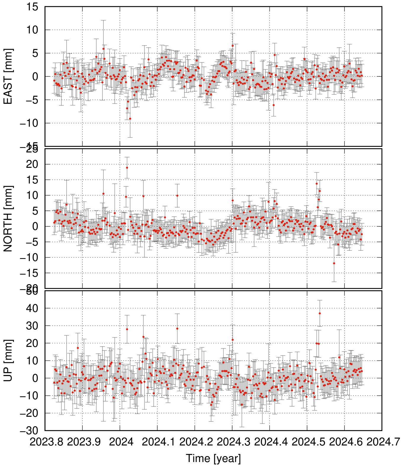
GJFV residual time series (some major events removed as well)
