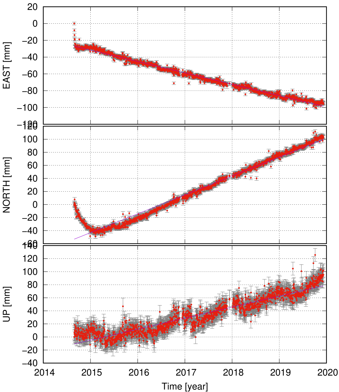
GJAC (64.83, -17.61) time series (ITRF 2014) v_e = -13.58 \pm 0.47 ; v_n = 28.94 \pm 1.66 ; v_u = 16.86 \pm 1.80 mm/yr
