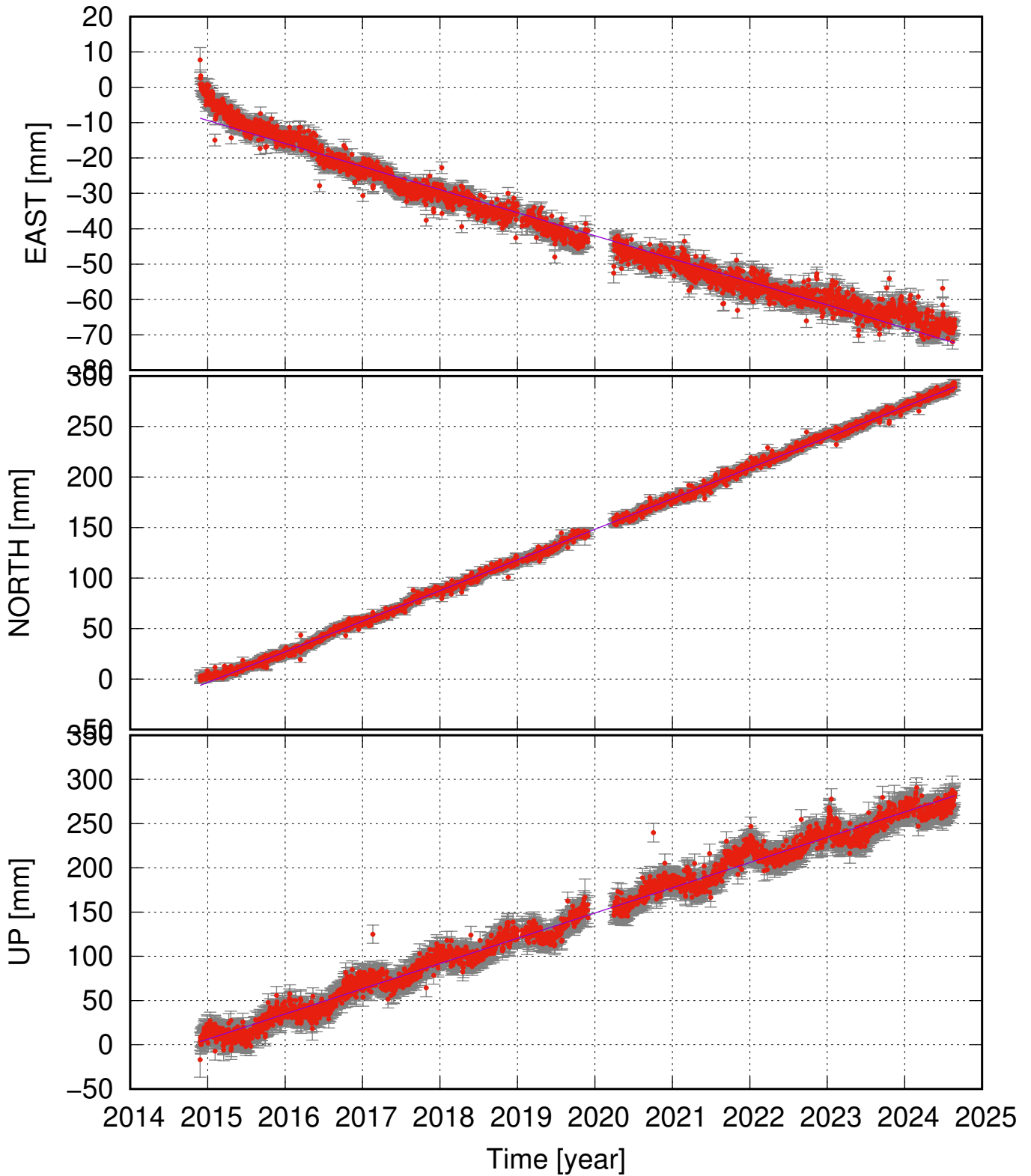
GIGO (64.84, -17.02) time series (ITRF 2014) v_e = -6.52 \pm 0.29 ; v_n = 30.34 \pm 0.27 ; v_u = 28.54 \pm 0.94 mm/yr
