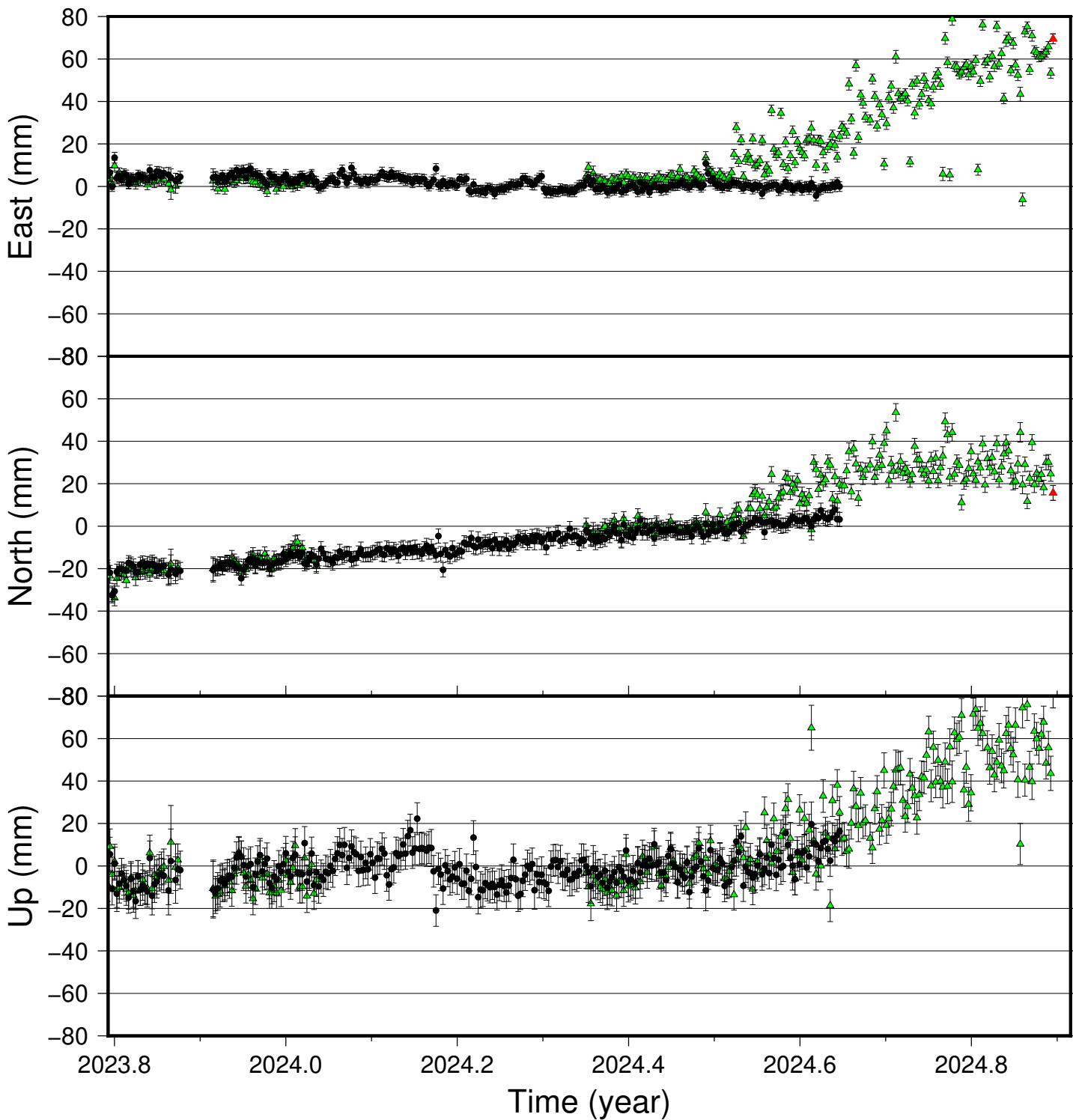
GIGO time series (IGS 2014), last 400 days
