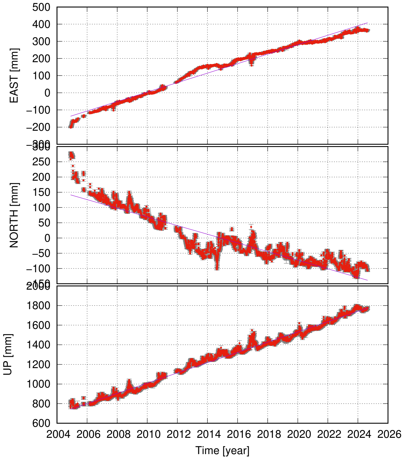
GFUM (64.41, -17.27) time series (ITRF 2014) ve = 27.59 +- 1.11; vn = -14.18 +- 1.64; vu = 52.27 +- 1.65 mm/yr
