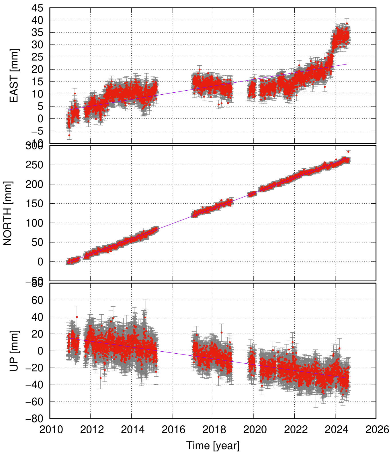
GFEL (63.95, -21.53) time series (ITRF 2014) v_e = 1.36 \pm 0.31 ; v_n = 19.73 \pm 0.23 ; v_u = -3.45 \pm 0.54 mm/yr
