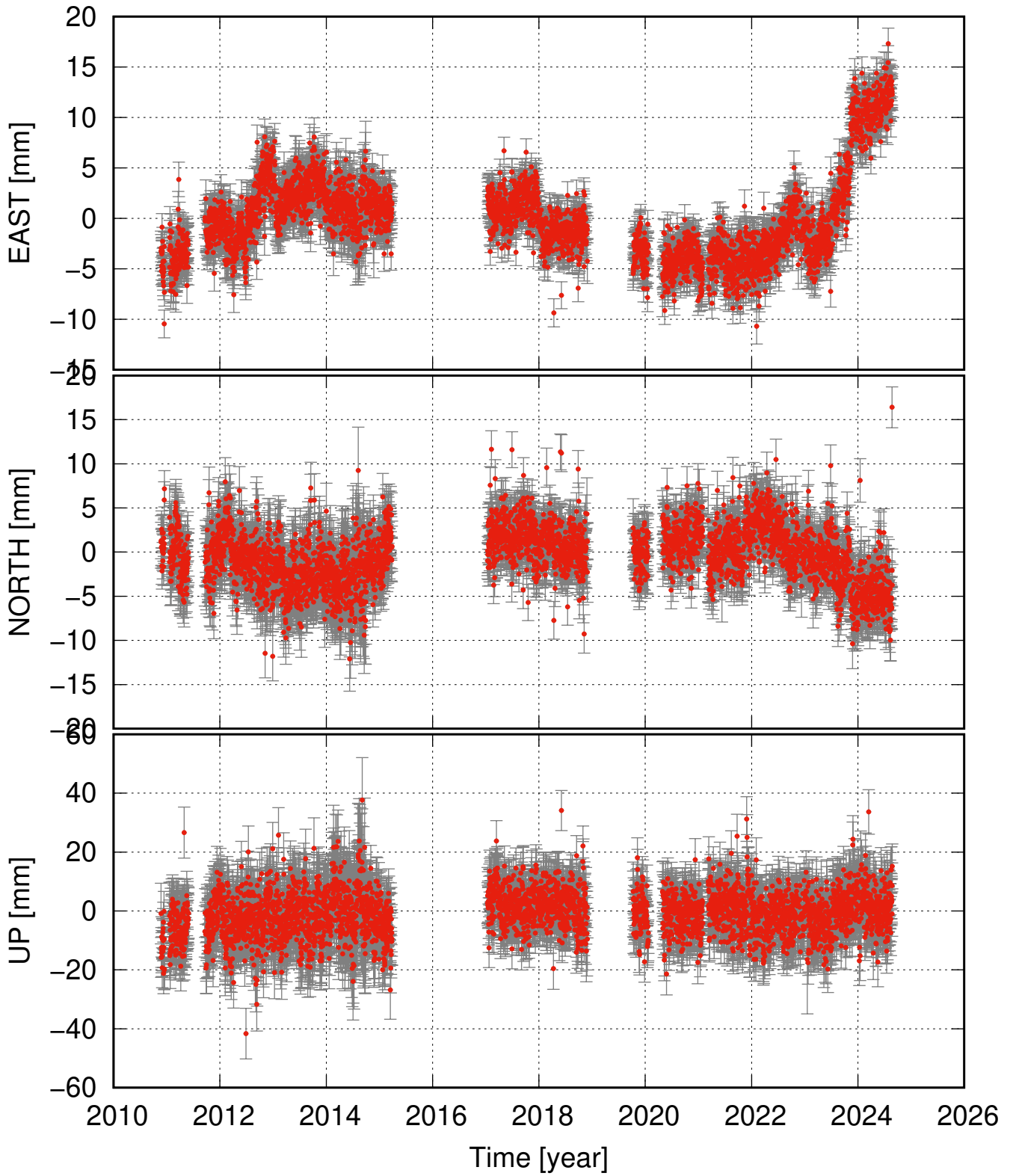
GFEL detrended and seasonal signal removed
