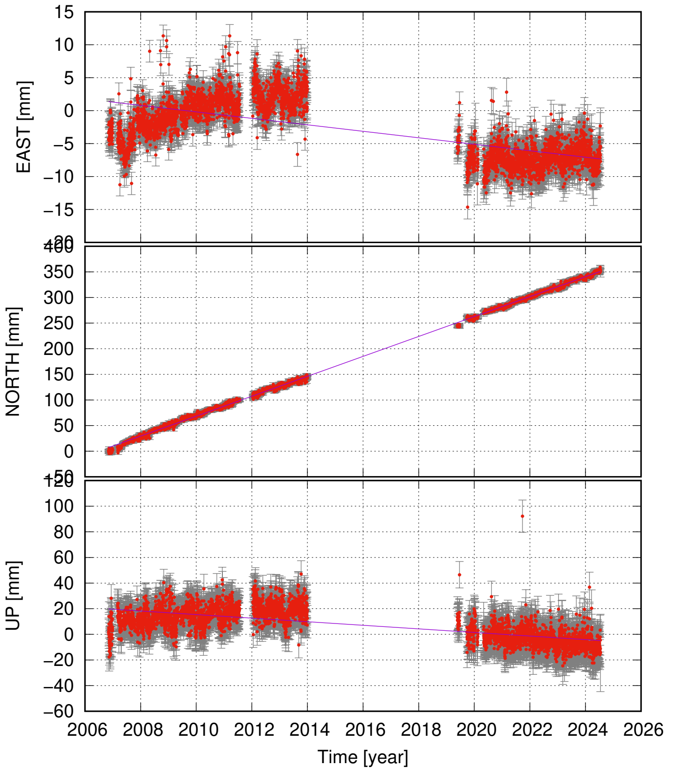
GAKE (66.08, -16.76) time series (ITRF 2014) v_e = -0.49 \pm 0.18 ; v_n = 19.44 \pm 0.17 ; v_u = -1.40 \pm 0.49 mm/yr
