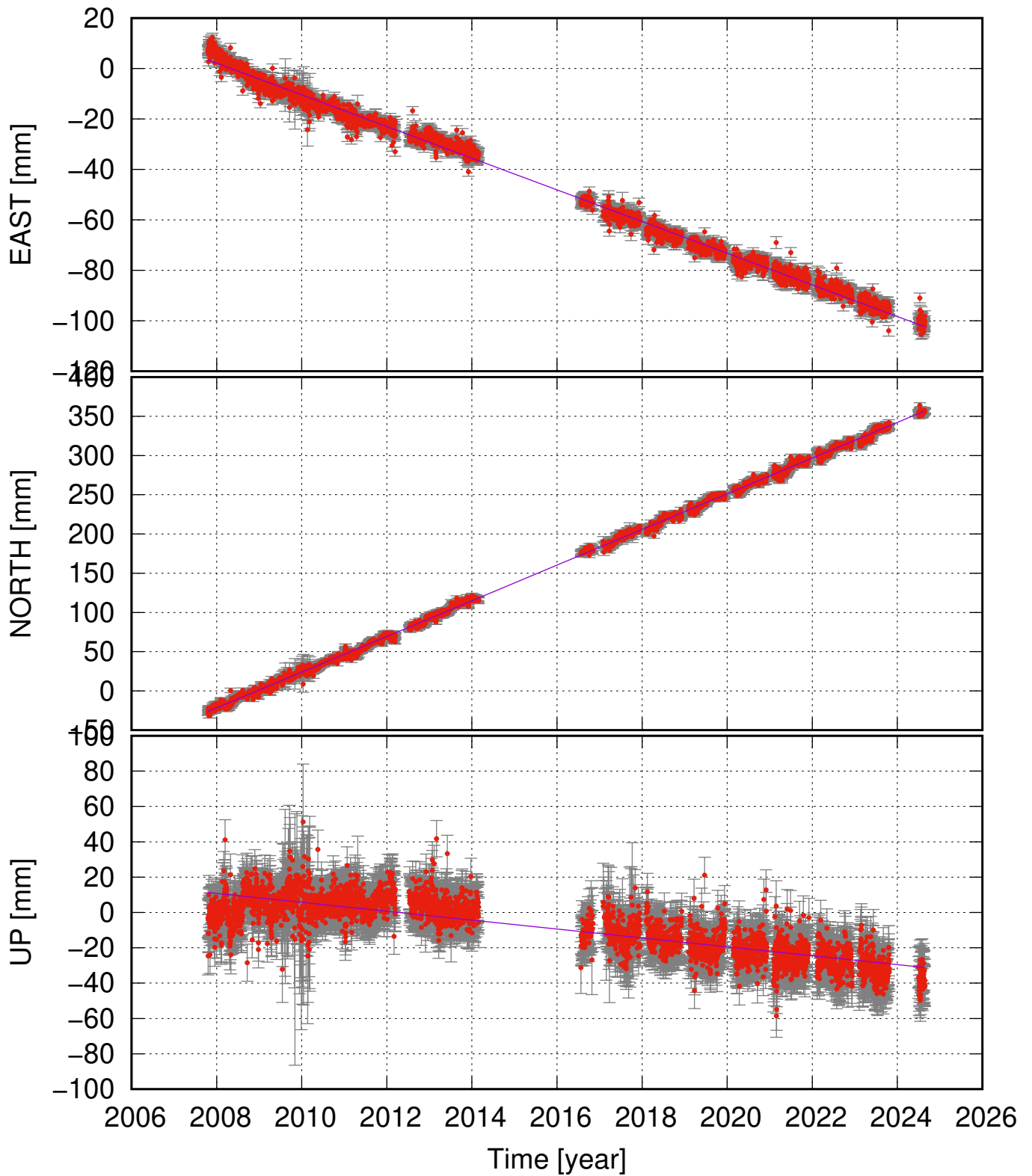
FTEY (66.16, -17.85) time series (ITRF 2014) v_e = -6.28 \pm 0.13 ; v_n = 22.73 \pm 0.18 ; v_u = -2.52 \pm 0.48 mm/yr
