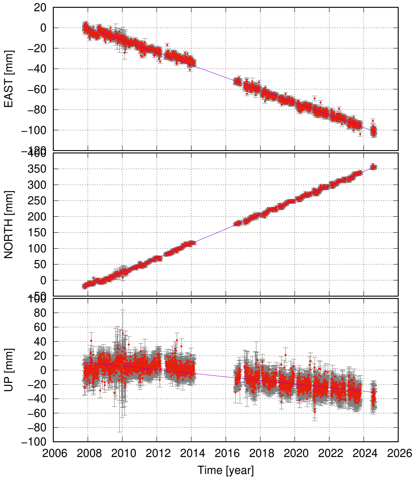
FTEY (66.16, -17.85) time series (ITRF 2014) v_e = -6.11 \pm 0.14 ; v_n = 22.58 \pm 0.21 ; v_u = -2.52 \pm 0.48 mm/yr
