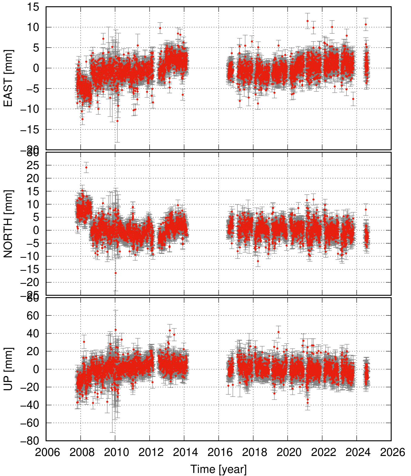
FTEY detrended and seasonal signal removed
